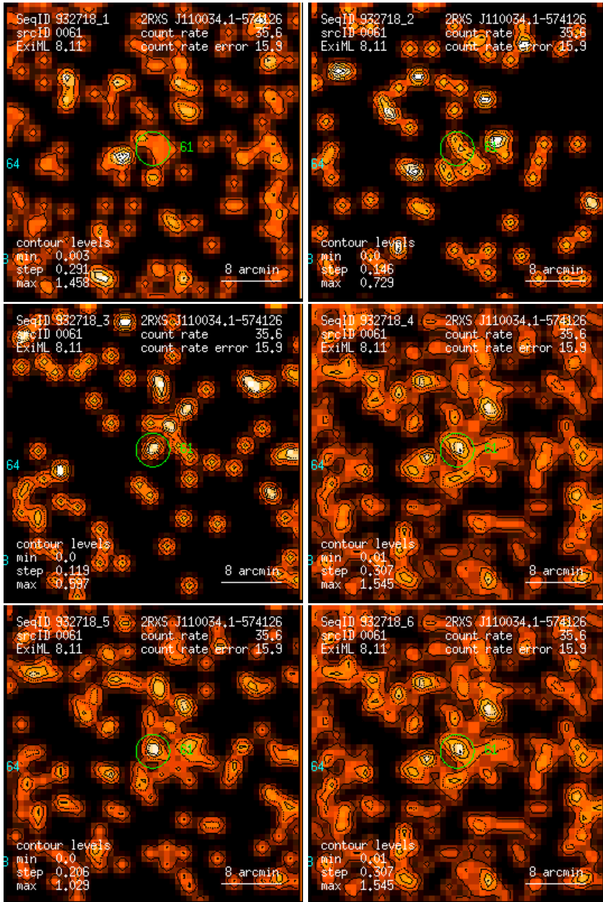
Figure 61: RASS 932718: detection 0061: band rate images, Gaussian filter: (1) PSPC channels 11 – 41, (2) 52 – 90, (3) 91 – 201, (4) 11 – 235, (5) 52 – 201, (6) 11 – 201. Broad band rates in counts/ks. Band rate contour levels in counts/ks/arcmin 2 .
