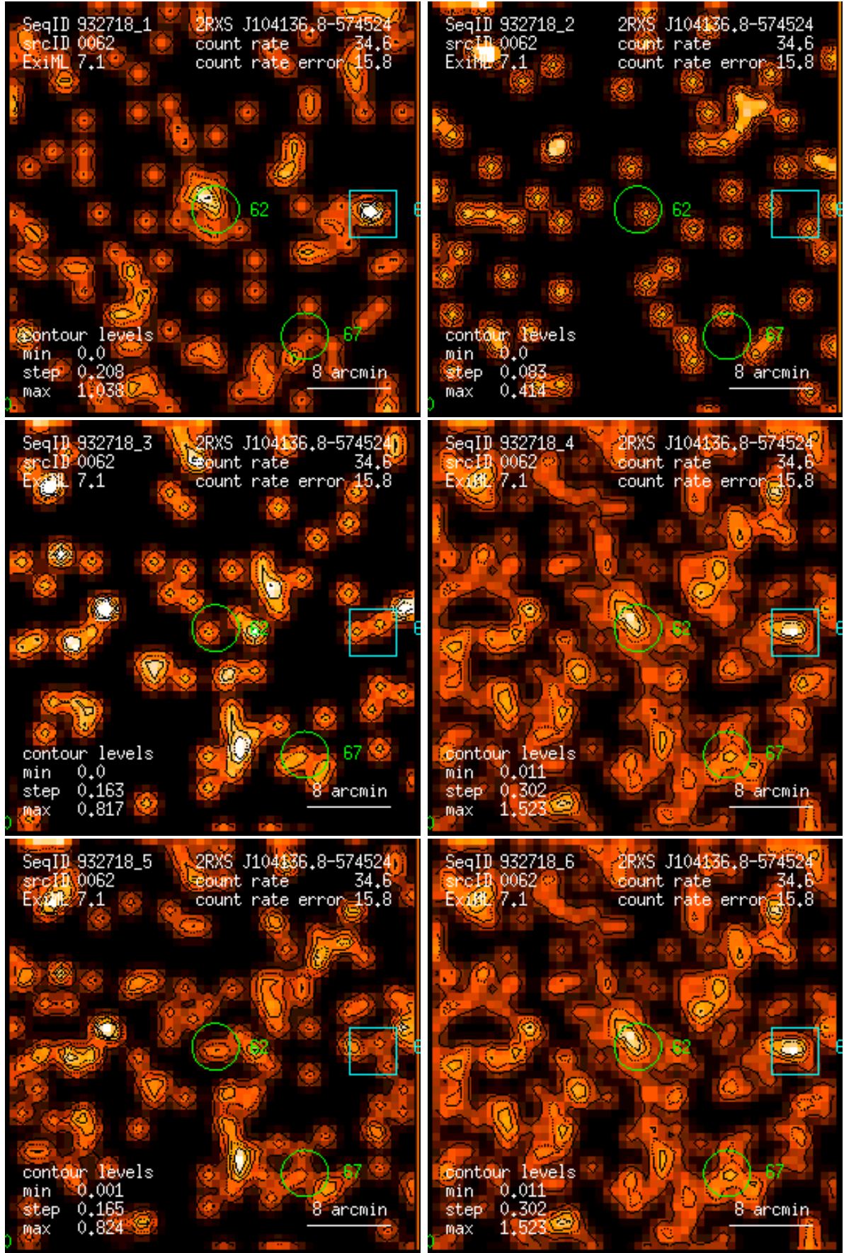
Figure 62: RASS 932718: detection 0062: band rate images, Gaussian filter: (1) PSPC channels 11 – 41, (2) 52 – 90, (3) 91 – 201, (4) 11 – 235, (5) 52 – 201, (6) 11 – 201. Broad band rates in counts/ks. Band rate contour levels in counts/ks/arcmin 2 .
