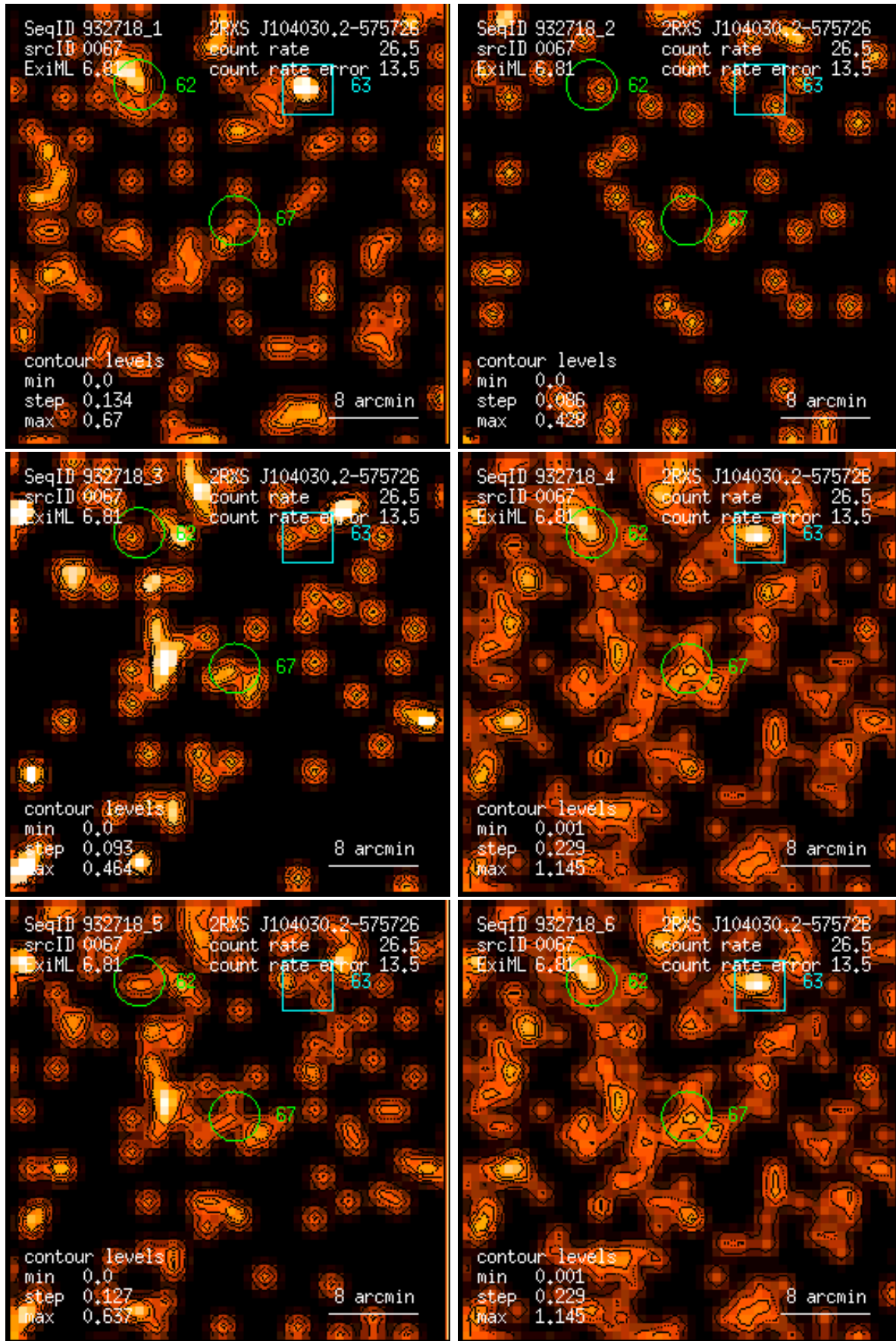
Figure 67: RASS 932718: detection 0067: band rate images, Gaussian filter: (1) PSPC channels 11 – 41, (2) 52 – 90, (3) 91 – 201, (4) 11 – 235, (5) 52 – 201, (6) 11 – 201. Broad band rates in counts/ks. Band rate contour levels in counts/ks/arcmin 2 .
