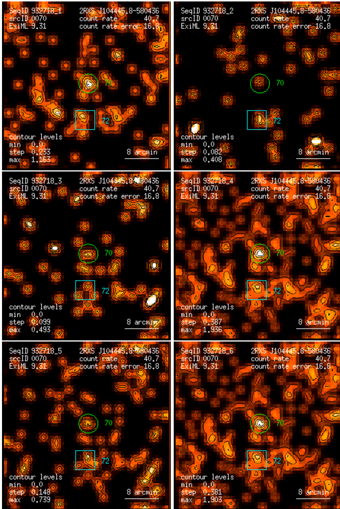
Figure 70: RASS 932718: detection 0070: band rate images, Gaussian filter: (1) PSPC channels 11 – 41, (2) 52 – 90, (3) 91 – 201, (4) 11 – 235, (5) 52 – 201, (6) 11 – 201. Broad band rates in counts/ks. Band rate contour levels in counts/ks/arcmin 2 .
