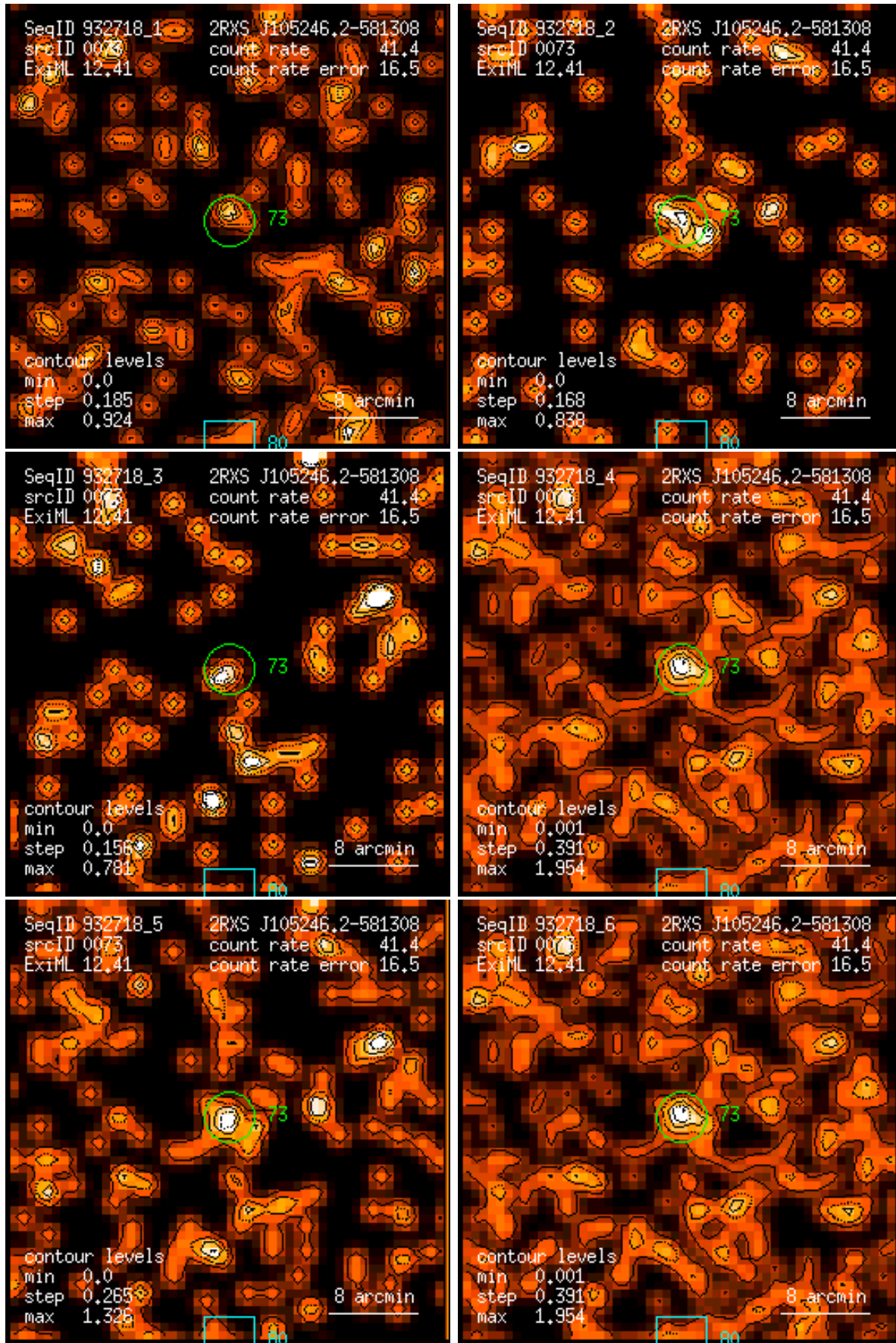
Figure 73: RASS 932718: detection 0073: band rate images, Gaussian filter: (1) PSPC channels 11 – 41, (2) 52 – 90, (3) 91 – 201, (4) 11 – 235, (5) 52 – 201, (6) 11 – 201. Broad band rates in counts/ks. Band rate contour levels in counts/ks/arcmin 2 .
