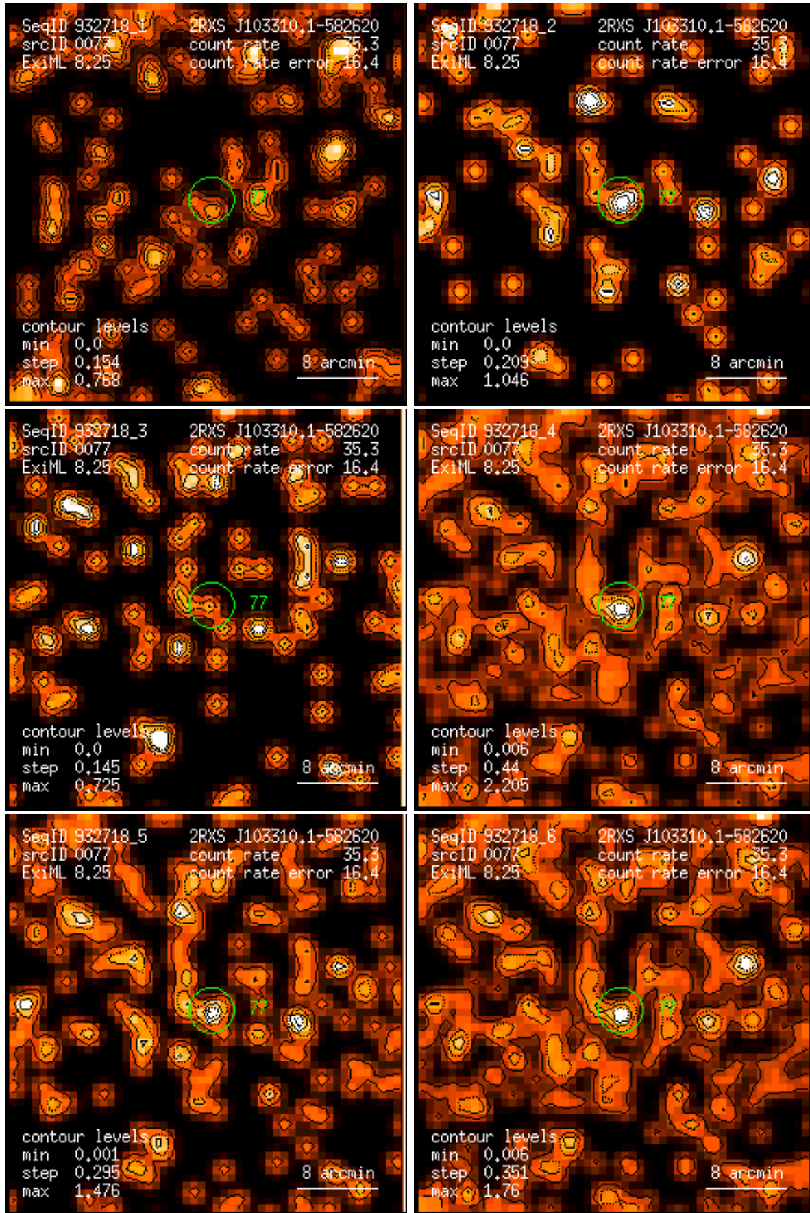
Figure 77: RASS 932718: detection 0077: band rate images, Gaussian filter: (1) PSPC channels 11 – 41, (2) 52 – 90, (3) 91 – 201, (4) 11 – 235, (5) 52 – 201, (6) 11 – 201. Broad band rates in counts/ks. Band rate contour levels in counts/ks/arcmin 2 .
