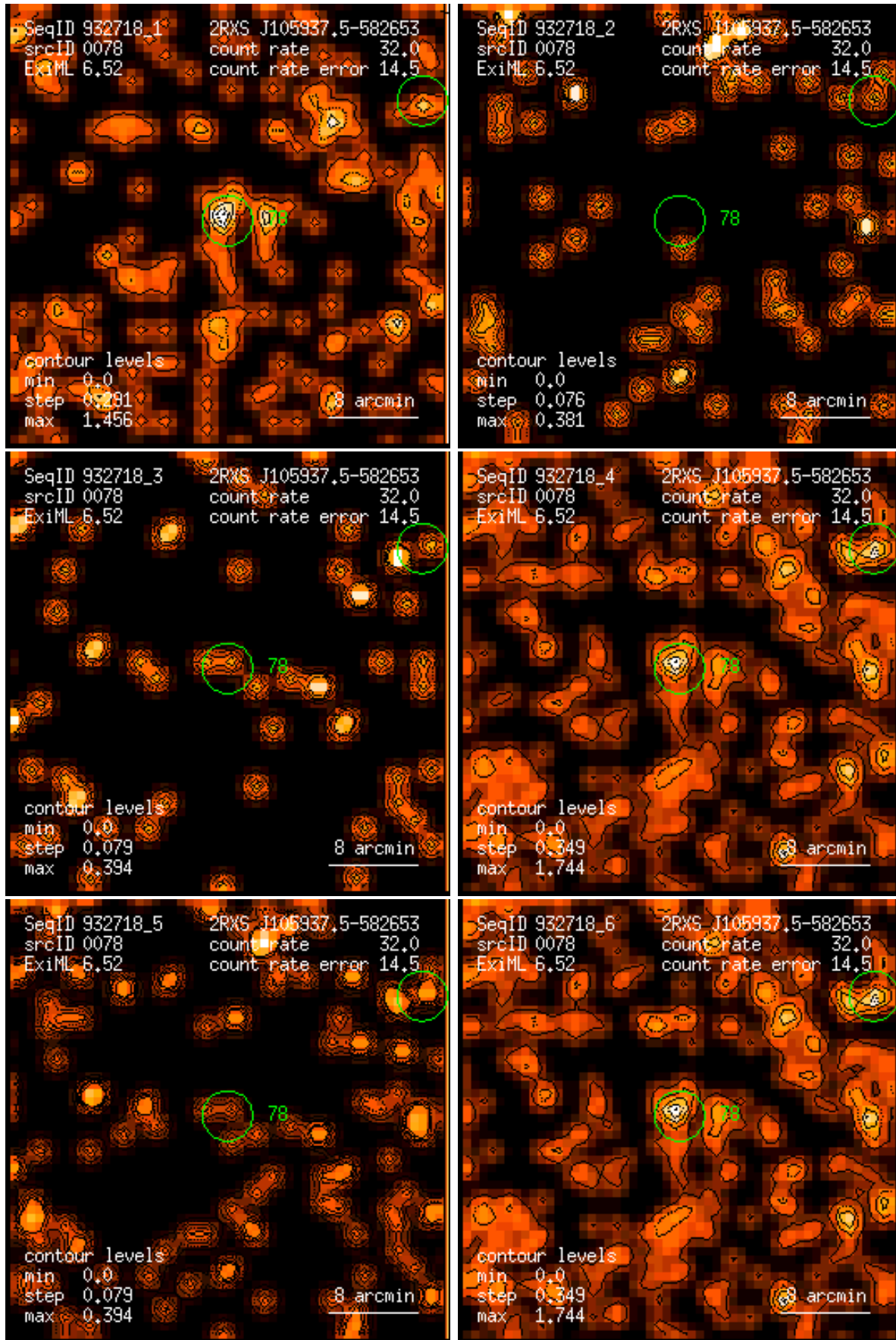
Figure 78: RASS 932718: detection 0078: band rate images, Gaussian filter: (1) PSPC channels 11 – 41, (2) 52 – 90, (3) 91 – 201, (4) 11 – 235, (5) 52 – 201, (6) 11 – 201. Broad band rates in counts/ks. Band rate contour levels in counts/ks/arcmin 2 .
