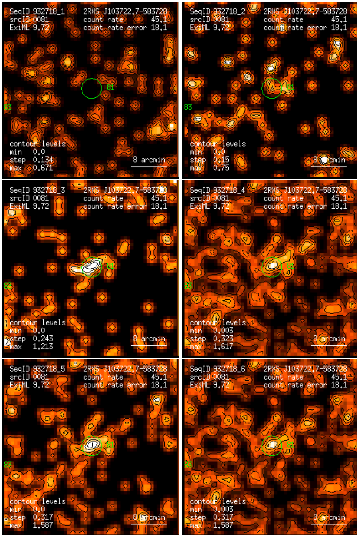
Figure 81: RASS 932718: detection 0081: band rate images, Gaussian filter: (1) PSPC channels 11 – 41, (2) 52 – 90, (3) 91 – 201, (4) 11 – 235, (5) 52 – 201, (6) 11 – 201. Broad band rates in counts/ks. Band rate contour levels in counts/ks/arcmin 2 .
