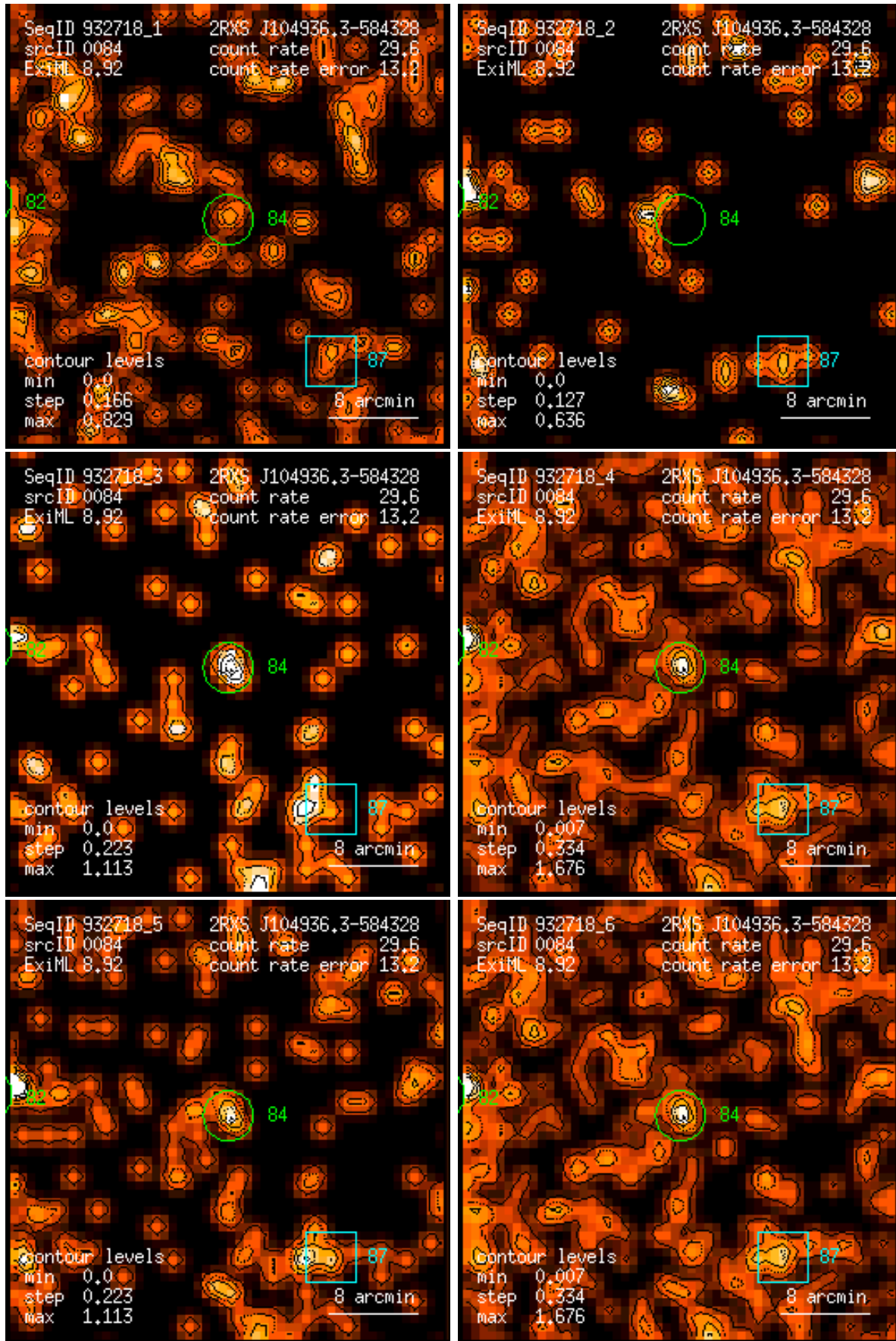
Figure 84: RASS 932718: detection 0084: band rate images, Gaussian filter: (1) PSPC channels 11 – 41, (2) 52 – 90, (3) 91 – 201, (4) 11 – 235, (5) 52 – 201, (6) 11 – 201. Broad band rates in counts/ks. Band rate contour levels in counts/ks/arcmin 2 .
