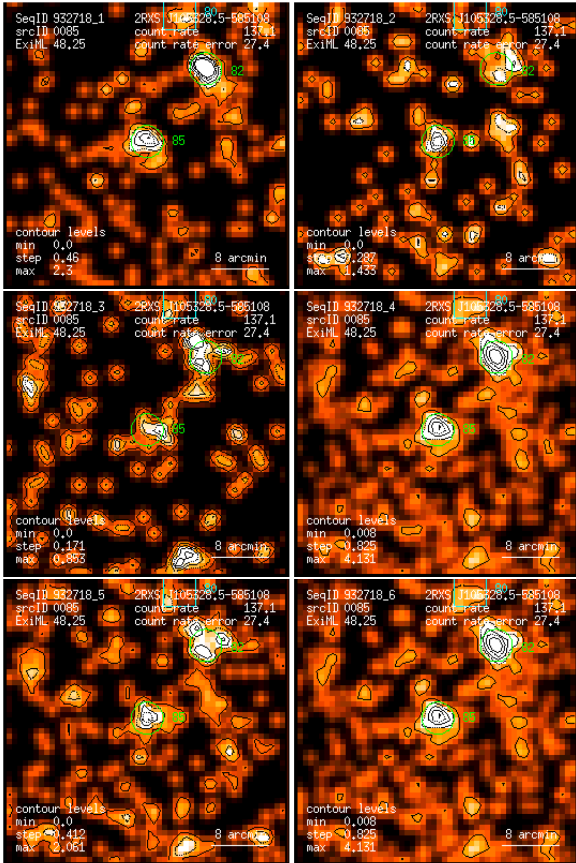
Figure 85: RASS 932718: detection 0085: band rate images, Gaussian filter: (1) PSPC channels 11 – 41, (2) 52 – 90, (3) 91 – 201, (4) 11 – 235, (5) 52 – 201, (6) 11 – 201. Broad band rates in counts/ks. Band rate contour levels in counts/ks/arcmin 2 .
