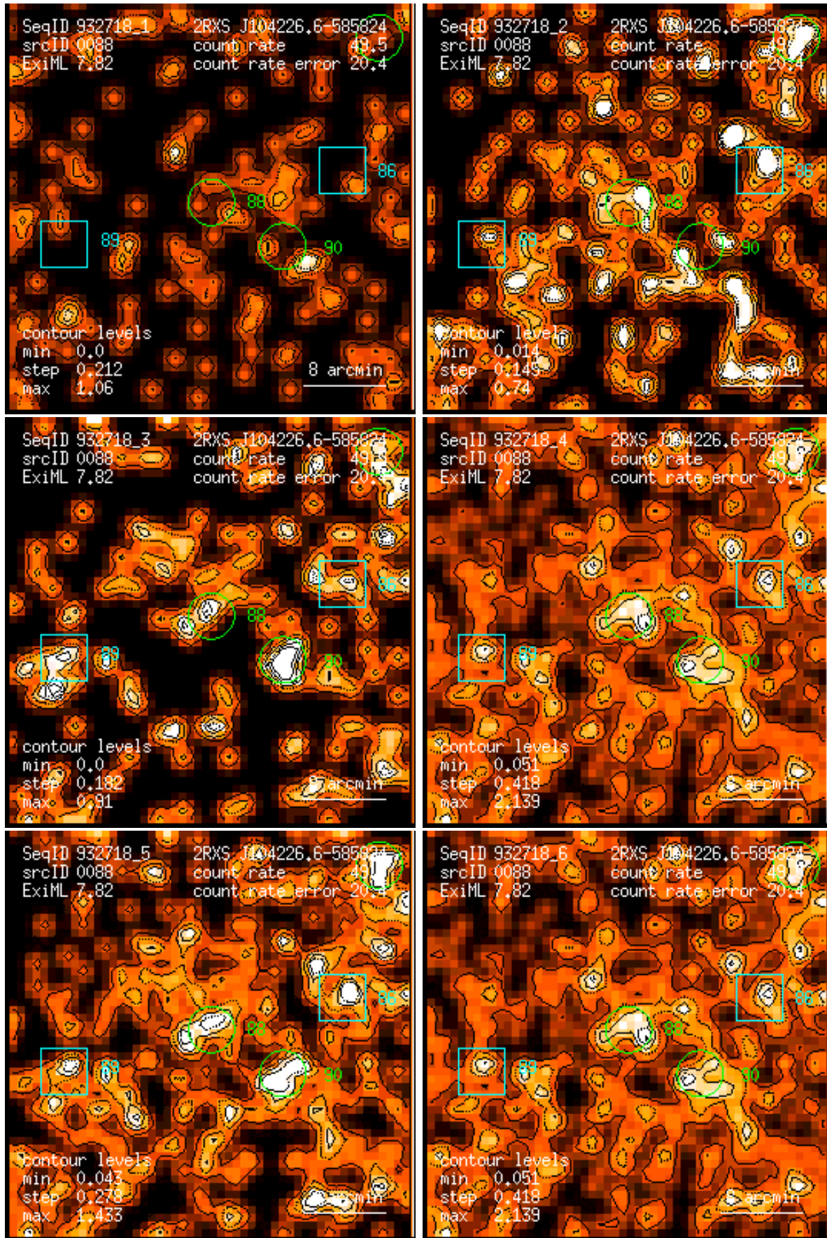
Figure 88: RASS 932718: detection 0088: band rate images, Gaussian filter: (1) PSPC channels 11 – 41, (2) 52 – 90, (3) 91 – 201, (4) 11 – 235, (5) 52 – 201, (6) 11 – 201. Broad band rates in counts/ks. Band rate contour levels in counts/ks/arcmin 2 .
