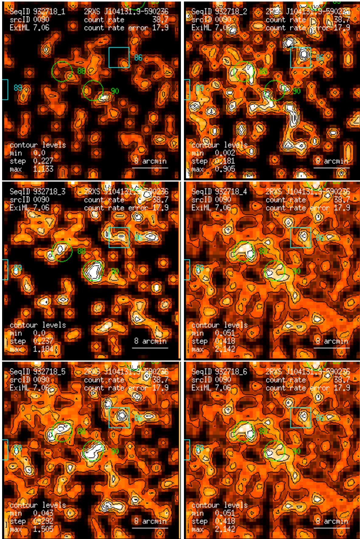
Figure 90: RASS 932718: detection 0090: band rate images, Gaussian filter: (1) PSPC channels 11 – 41, (2) 52 – 90, (3) 91 – 201, (4) 11 – 235, (5) 52 – 201, (6) 11 – 201. Broad band rates in counts/ks. Band rate contour levels in counts/ks/arcmin 2 .
