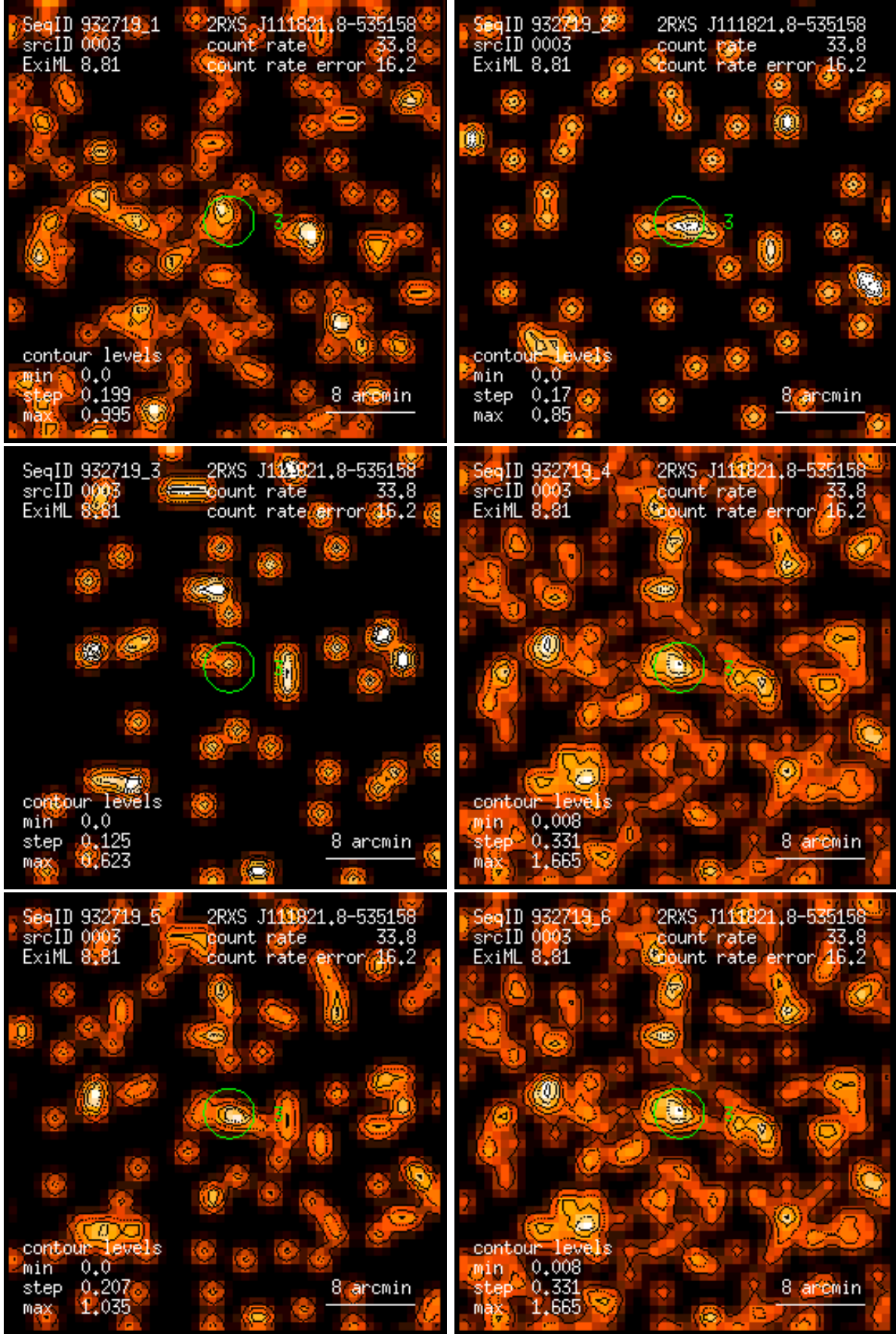
Figure 3: RASS 932719: detection 0003: band rate images, Gaussian filter: (1) PSPC channels 11 – 41, (2) 52 – 90, (3) 91 – 201, (4) 11 – 235, (5) 52 – 201, (6) 11 – 201. Broad band rates in counts/ks. Band rate contour levels in counts/ks/arcmin 2 .
