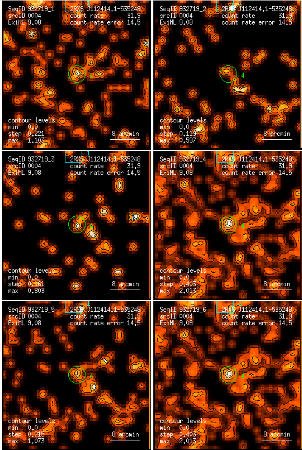
Figure 4: RASS 932719: detection 0004: band rate images, Gaussian filter: (1) PSPC channels 11 – 41, (2) 52 – 90, (3) 91 – 201, (4) 11 – 235, (5) 52 – 201, (6) 11 – 201. Broad band rates in counts/ks. Band rate contour levels in counts/ks/arcmin 2 .
