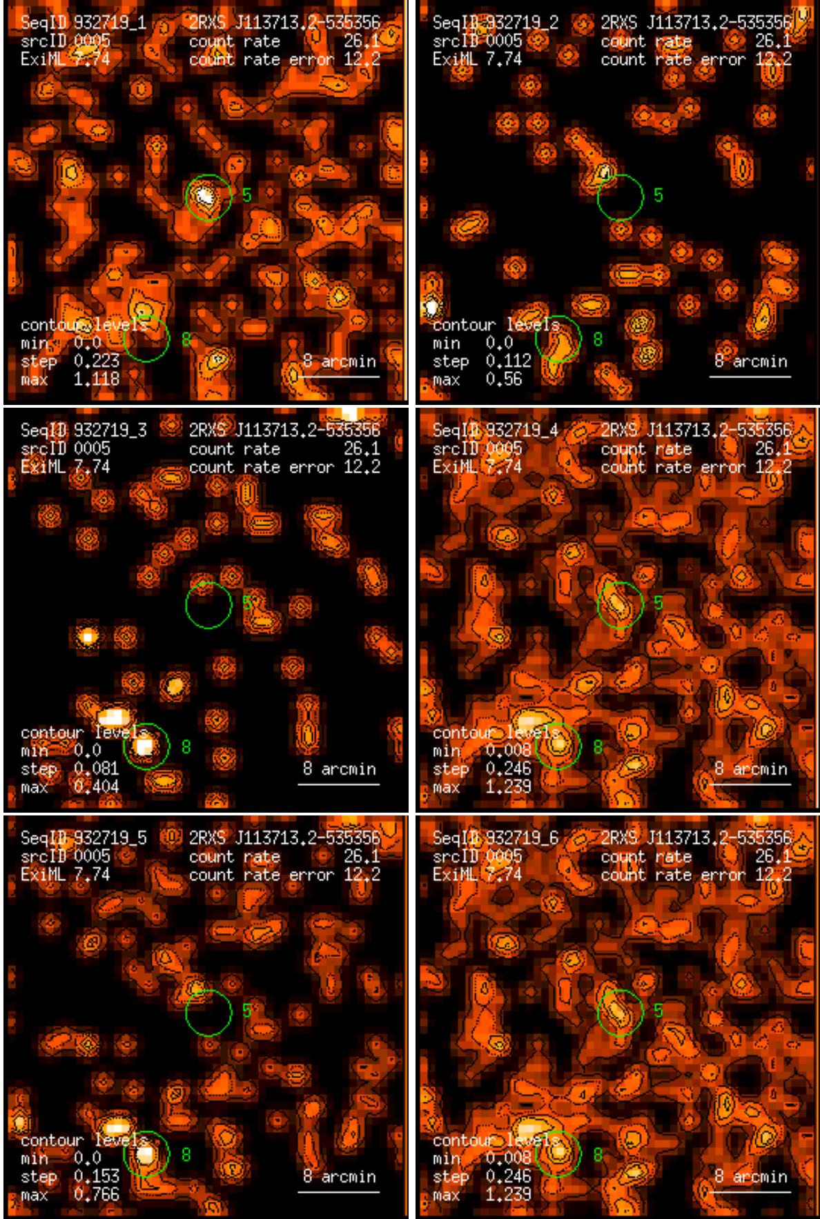
Figure 5: RASS 932719: detection 0005: band rate images, Gaussian filter: (1) PSPC channels 11 – 41, (2) 52 – 90, (3) 91 – 201, (4) 11 – 235, (5) 52 – 201, (6) 11 – 201. Broad band rates in counts/ks. Band rate contour levels in counts/ks/arcmin 2 .
