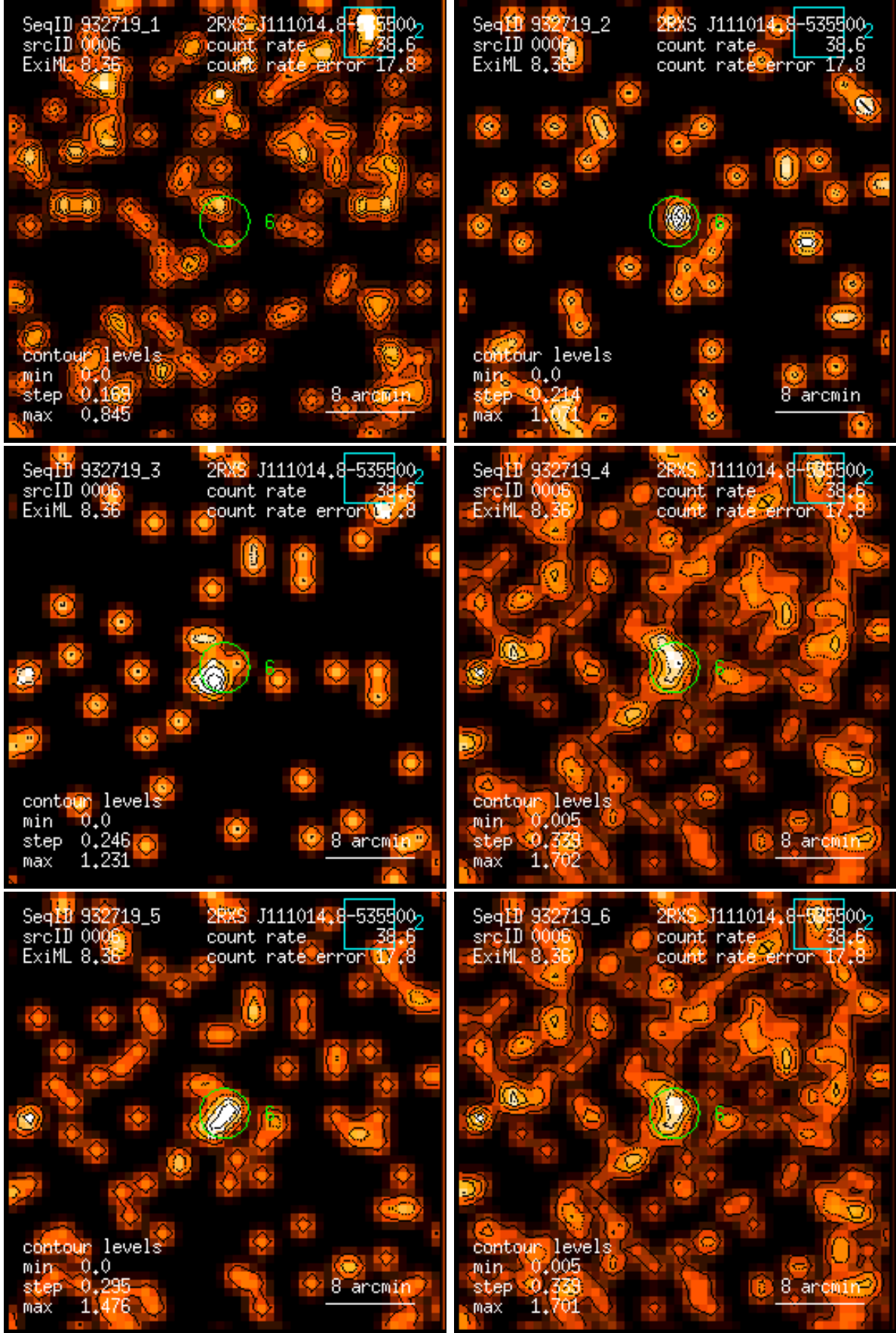
Figure 6: RASS 932719: detection 0006: band rate images, Gaussian filter: (1) PSPC channels 11 – 41, (2) 52 – 90, (3) 91 – 201, (4) 11 – 235, (5) 52 – 201, (6) 11 – 201. Broad band rates in counts/ks. Band rate contour levels in counts/ks/arcmin 2 .
