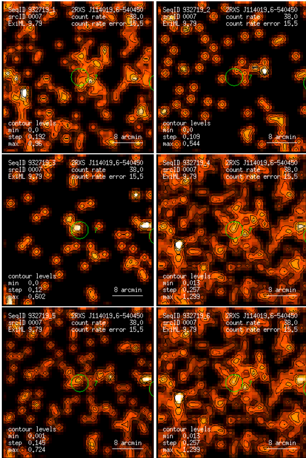
Figure 7: RASS 932719: detection 0007: band rate images, Gaussian filter: (1) PSPC channels 11 – 41, (2) 52 – 90, (3) 91 – 201, (4) 11 – 235, (5) 52 – 201, (6) 11 – 201. Broad band rates in counts/ks. Band rate contour levels in counts/ks/arcmin 2 .
