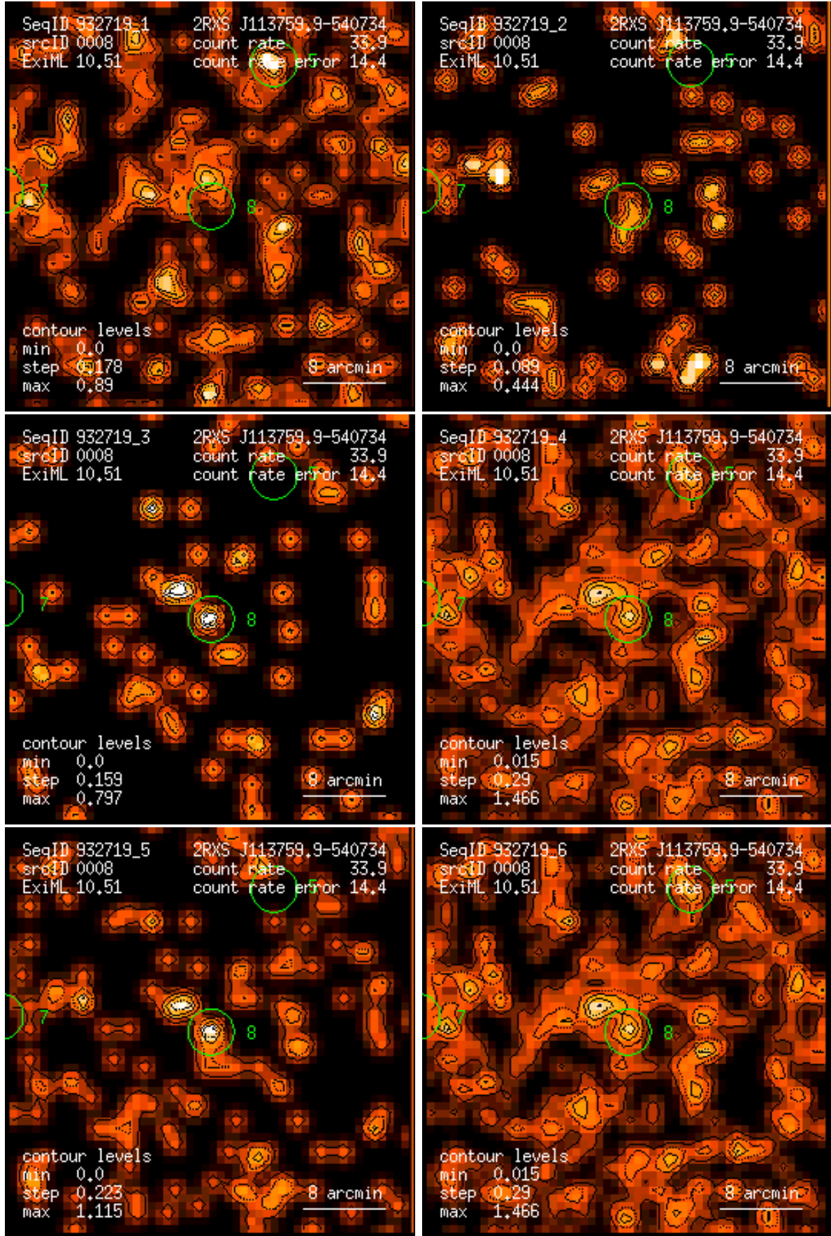
Figure 8: RASS 932719: detection 0008: band rate images, Gaussian filter: (1) PSPC channels 11 – 41, (2) 52 – 90, (3) 91 – 201, (4) 11 – 235, (5) 52 – 201, (6) 11 – 201. Broad band rates in counts/ks. Band rate contour levels in counts/ks/arcmin 2 .
