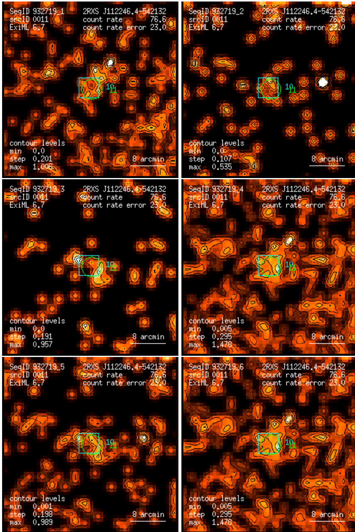
Figure 11: RASS 932719: detection 0011: band rate images, Gaussian filter: (1) PSPC channels 11 – 41, (2) 52 – 90, (3) 91 – 201, (4) 11 – 235, (5) 52 – 201, (6) 11 – 201. Broad band rates in counts/ks. Band rate contour levels in counts/ks/arcmin 2 .
