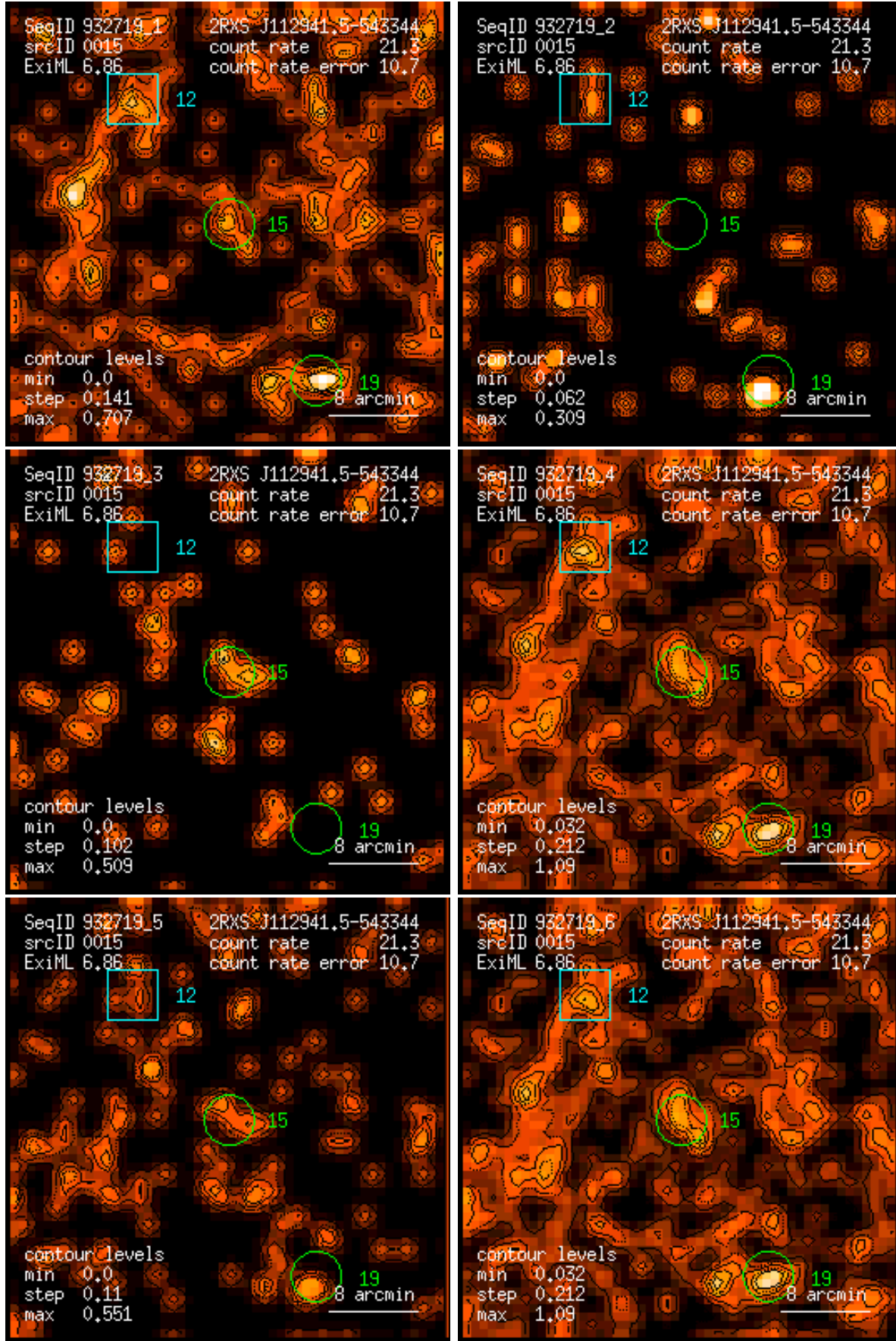
Figure 15: RASS 932719: detection 0015: band rate images, Gaussian filter: (1) PSPC channels 11 – 41, (2) 52 – 90, (3) 91 – 201, (4) 11 – 235, (5) 52 – 201, (6) 11 – 201. Broad band rates in counts/ks. Band rate contour levels in counts/ks/arcmin 2 .
