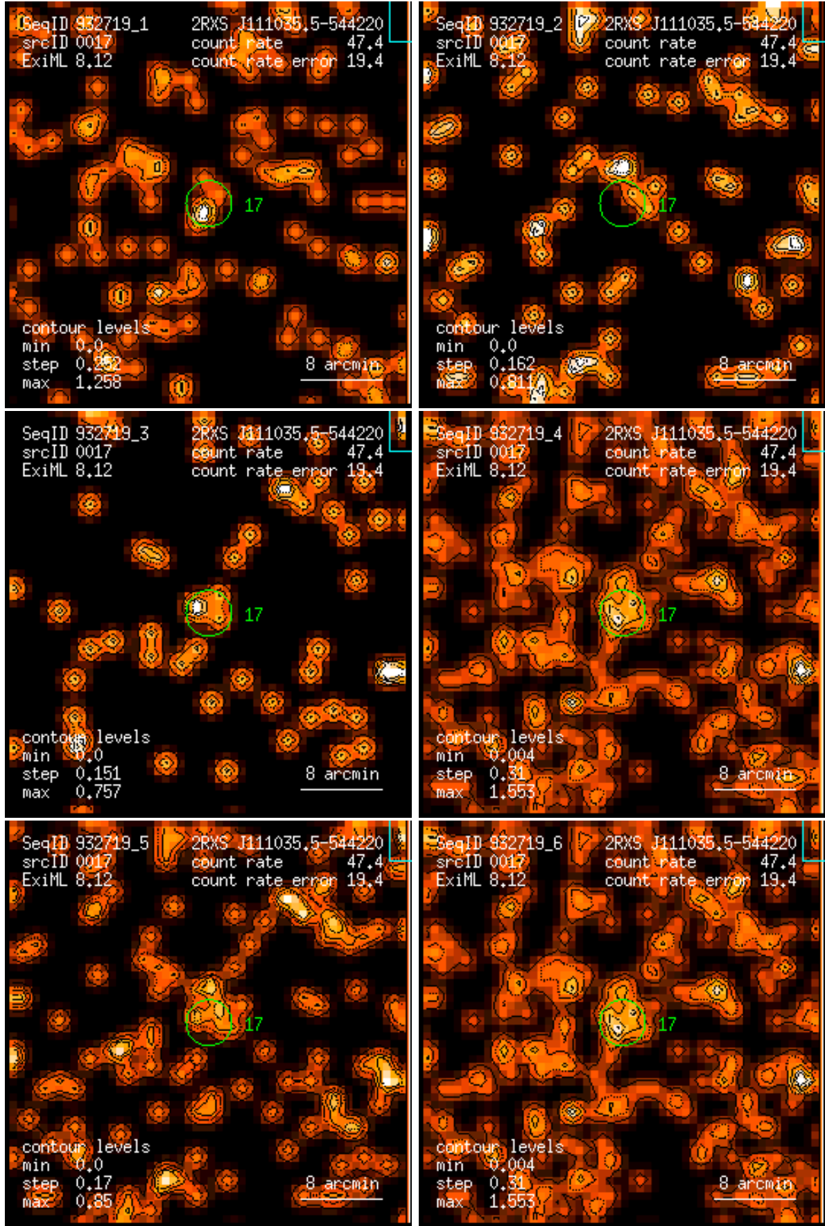
Figure 17: RASS 932719: detection 0017: band rate images, Gaussian filter: (1) PSPC channels 11 – 41, (2) 52 – 90, (3) 91 – 201, (4) 11 – 235, (5) 52 – 201, (6) 11 – 201. Broad band rates in counts/ks. Band rate contour levels in counts/ks/arcmin 2 .
