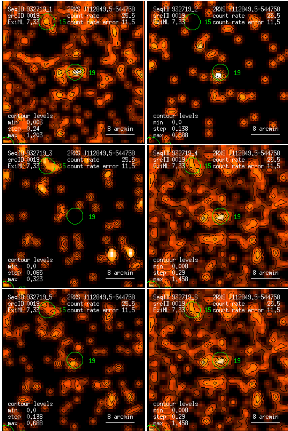
Figure 19: RASS 932719: detection 0019: band rate images, Gaussian filter: (1) PSPC channels 11 – 41, (2) 52 – 90, (3) 91 – 201, (4) 11 – 235, (5) 52 – 201, (6) 11 – 201. Broad band rates in counts/ks. Band rate contour levels in counts/ks/arcmin 2 .
