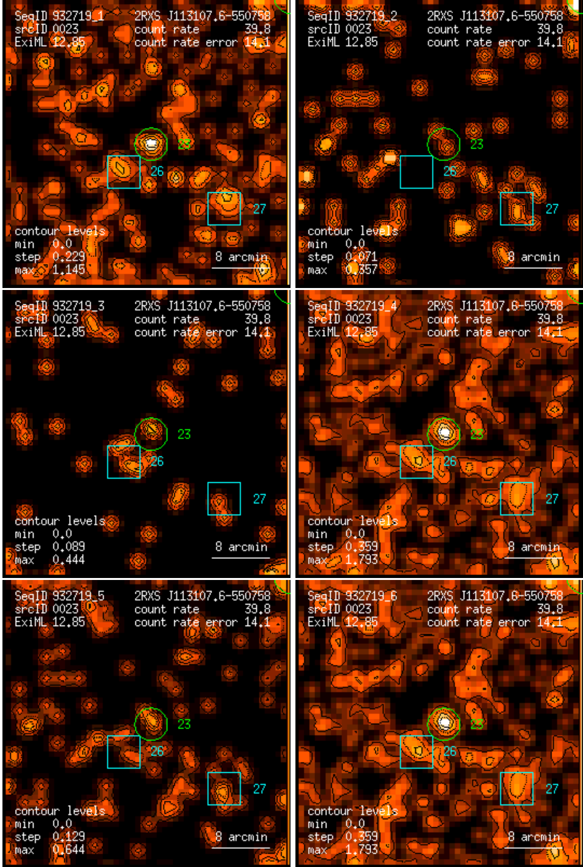
Figure 23: RASS 932719: detection 0023: band rate images, Gaussian filter: (1) PSPC channels 11 – 41, (2) 52 – 90, (3) 91 – 201, (4) 11 – 235, (5) 52 – 201, (6) 11 – 201. Broad band rates in counts/ks. Band rate contour levels in counts/ks/arcmin 2 .
