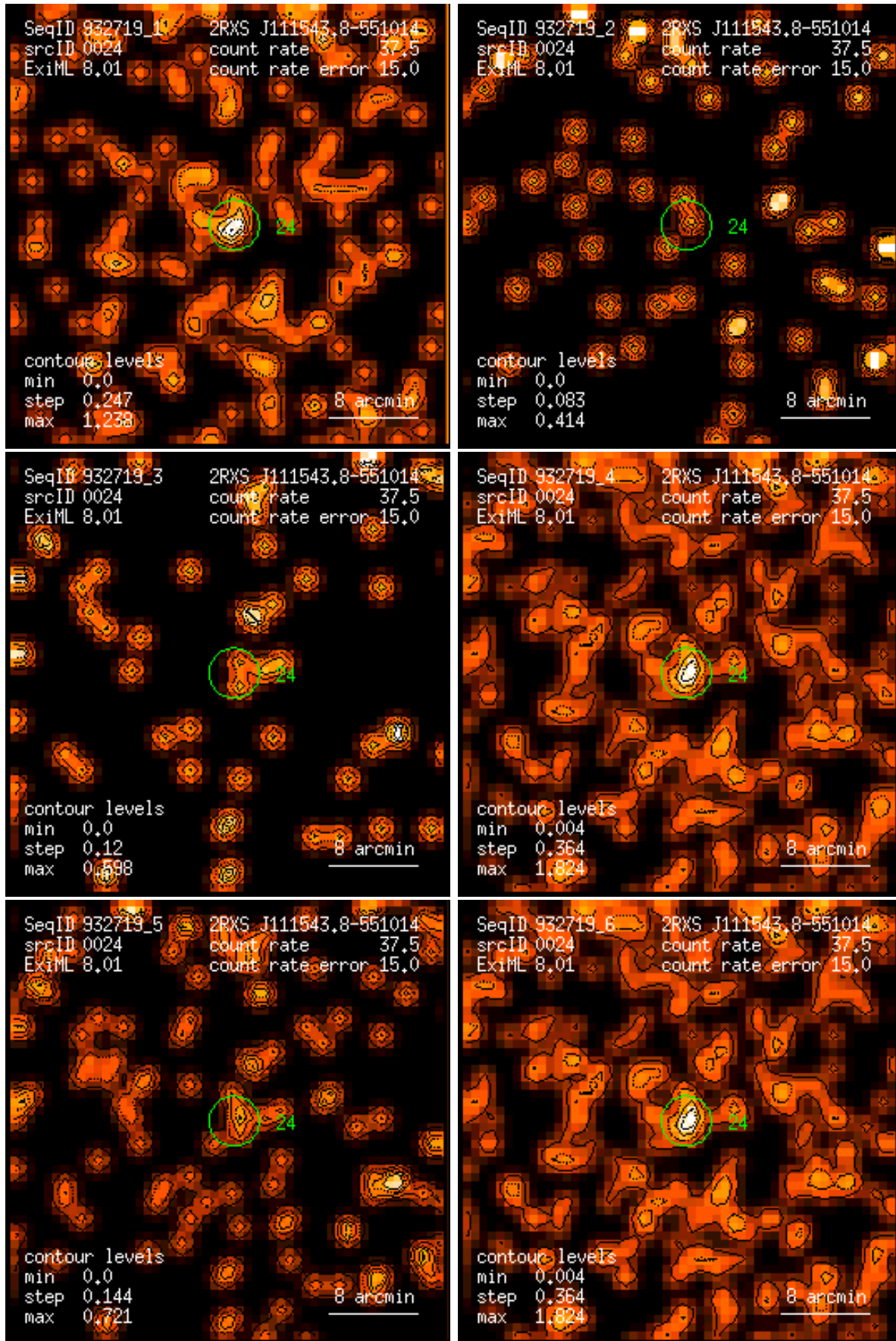
Figure 24: RASS 932719: detection 0024: band rate images, Gaussian filter: (1) PSPC channels 11 – 41, (2) 52 – 90, (3) 91 – 201, (4) 11 – 235, (5) 52 – 201, (6) 11 – 201. Broad band rates in counts/ks. Band rate contour levels in counts/ks/arcmin 2 .
