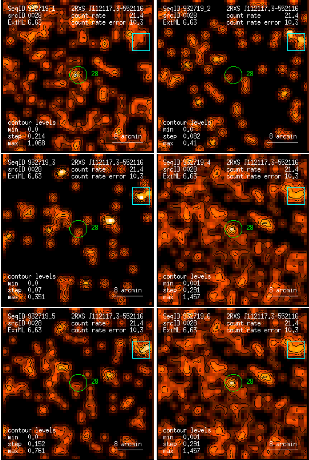
Figure 28: RASS 932719: detection 0028: band rate images, Gaussian filter: (1) PSPC channels 11 – 41, (2) 52 – 90, (3) 91 – 201, (4) 11 – 235, (5) 52 – 201, (6) 11 – 201. Broad band rates in counts/ks. Band rate contour levels in counts/ks/arcmin 2 .
