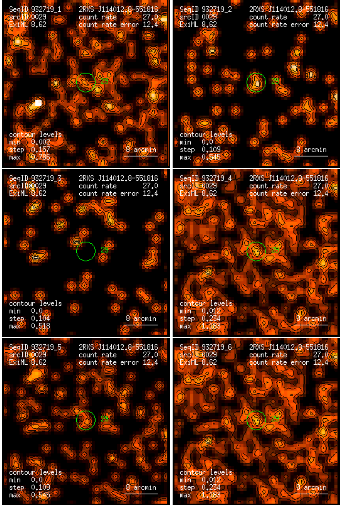
Figure 29: RASS 932719: detection 0029: band rate images, Gaussian filter: (1) PSPC channels 11 – 41, (2) 52 – 90, (3) 91 – 201, (4) 11 – 235, (5) 52 – 201, (6) 11 – 201. Broad band rates in counts/ks. Band rate contour levels in counts/ks/arcmin 2 .
