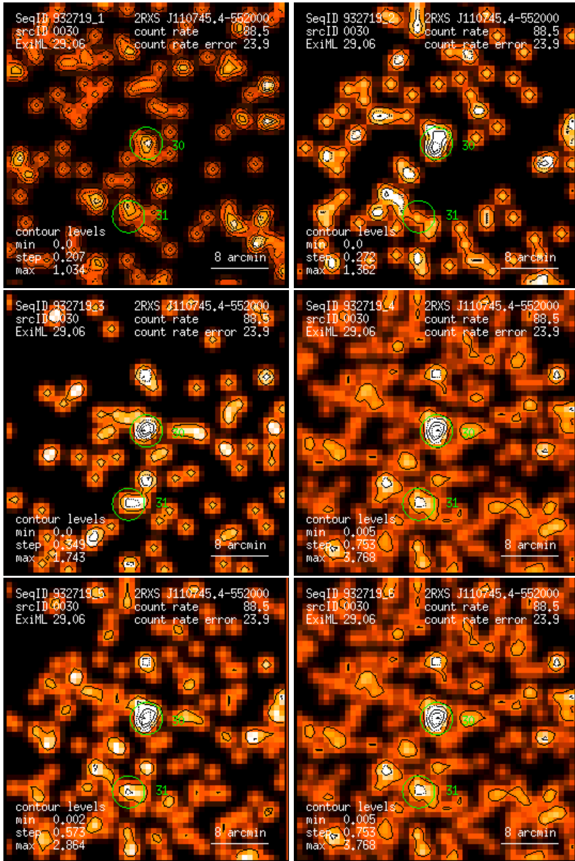
Figure 30: RASS 932719: detection 0030: band rate images, Gaussian filter: (1) PSPC channels 11 – 41, (2) 52 – 90, (3) 91 – 201, (4) 11 – 235, (5) 52 – 201, (6) 11 – 201. Broad band rates in counts/ks. Band rate contour levels in counts/ks/arcmin 2 .
