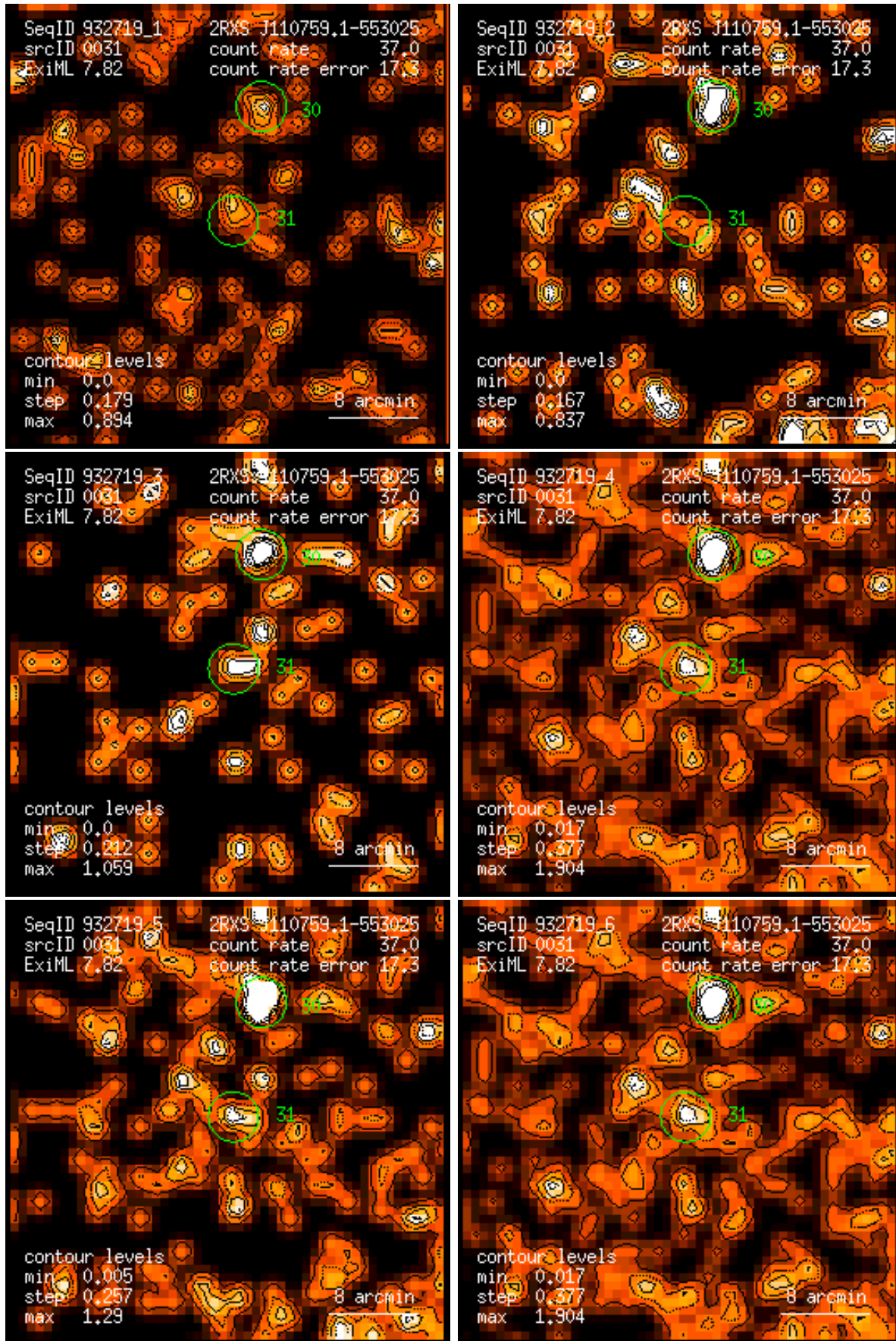
Figure 31: RASS 932719: detection 0031: band rate images, Gaussian filter: (1) PSPC channels 11 – 41, (2) 52 – 90, (3) 91 – 201, (4) 11 – 235, (5) 52 – 201, (6) 11 – 201. Broad band rates in counts/ks. Band rate contour levels in counts/ks/arcmin 2 .
