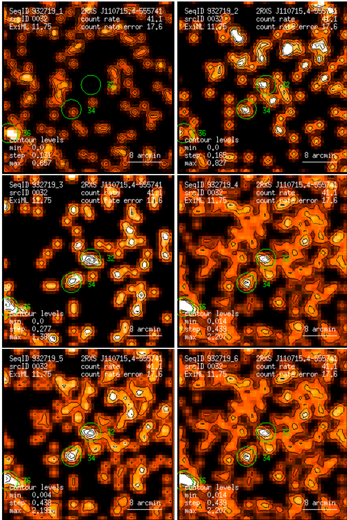
Figure 32: RASS 932719: detection 0032: band rate images, Gaussian filter: (1) PSPC channels 11 – 41, (2) 52 – 90, (3) 91 – 201, (4) 11 – 235, (5) 52 – 201, (6) 11 – 201. Broad band rates in counts/ks. Band rate contour levels in counts/ks/arcmin 2 .
