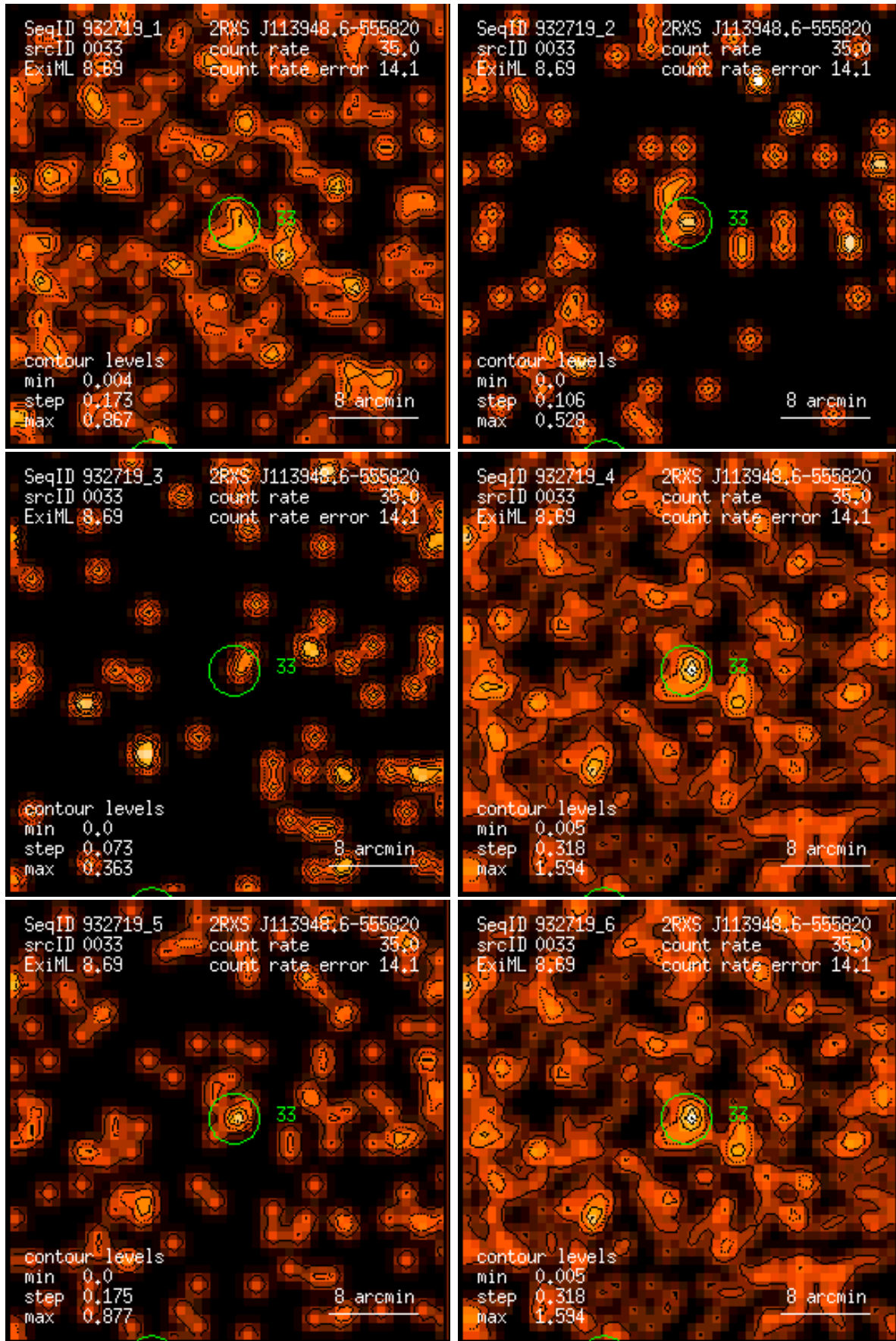
Figure 33: RASS 932719: detection 0033: band rate images, Gaussian filter: (1) PSPC channels 11 – 41, (2) 52 – 90, (3) 91 – 201, (4) 11 – 235, (5) 52 – 201, (6) 11 – 201. Broad band rates in counts/ks. Band rate contour levels in counts/ks/arcmin 2 .
