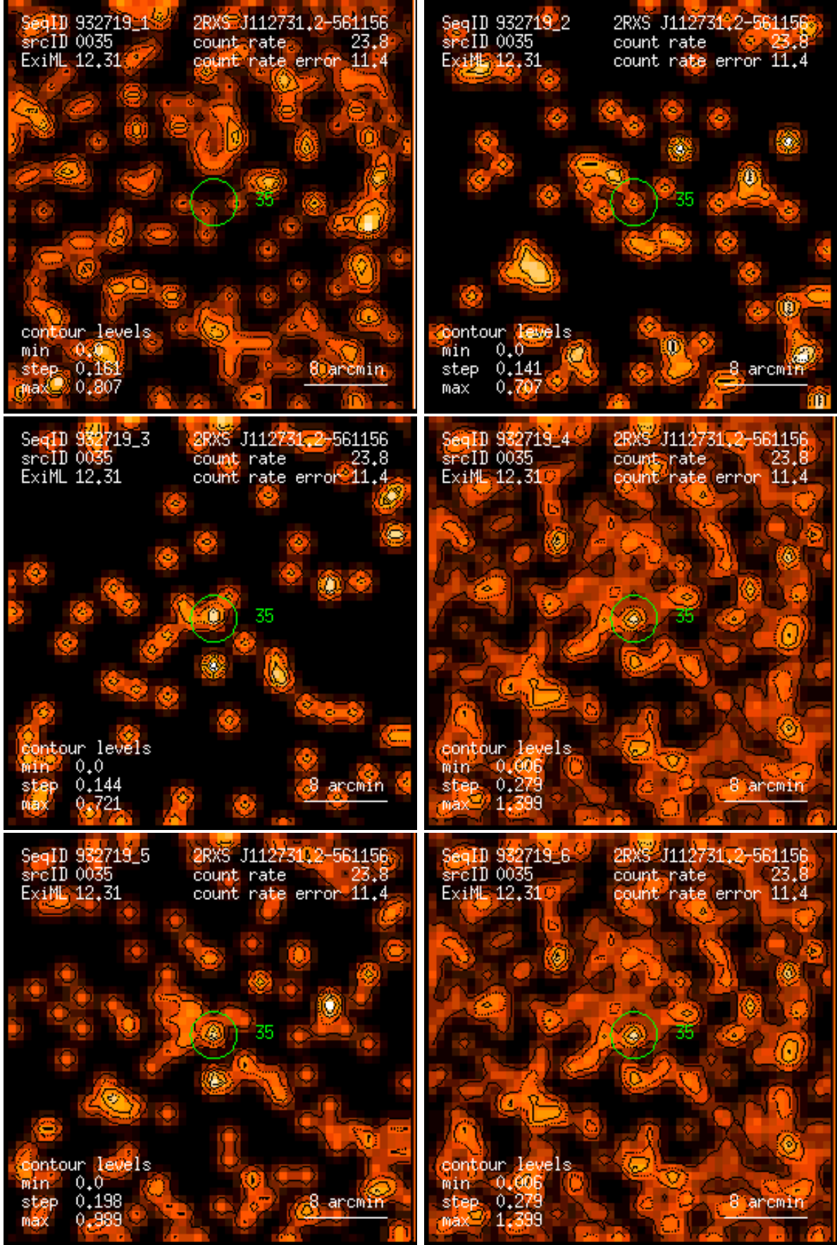
Figure 35: RASS 932719: detection 0035: band rate images, Gaussian filter: (1) PSPC channels 11 – 41, (2) 52 – 90, (3) 91 – 201, (4) 11 – 235, (5) 52 – 201, (6) 11 – 201. Broad band rates in counts/ks. Band rate contour levels in counts/ks/arcmin 2 .
