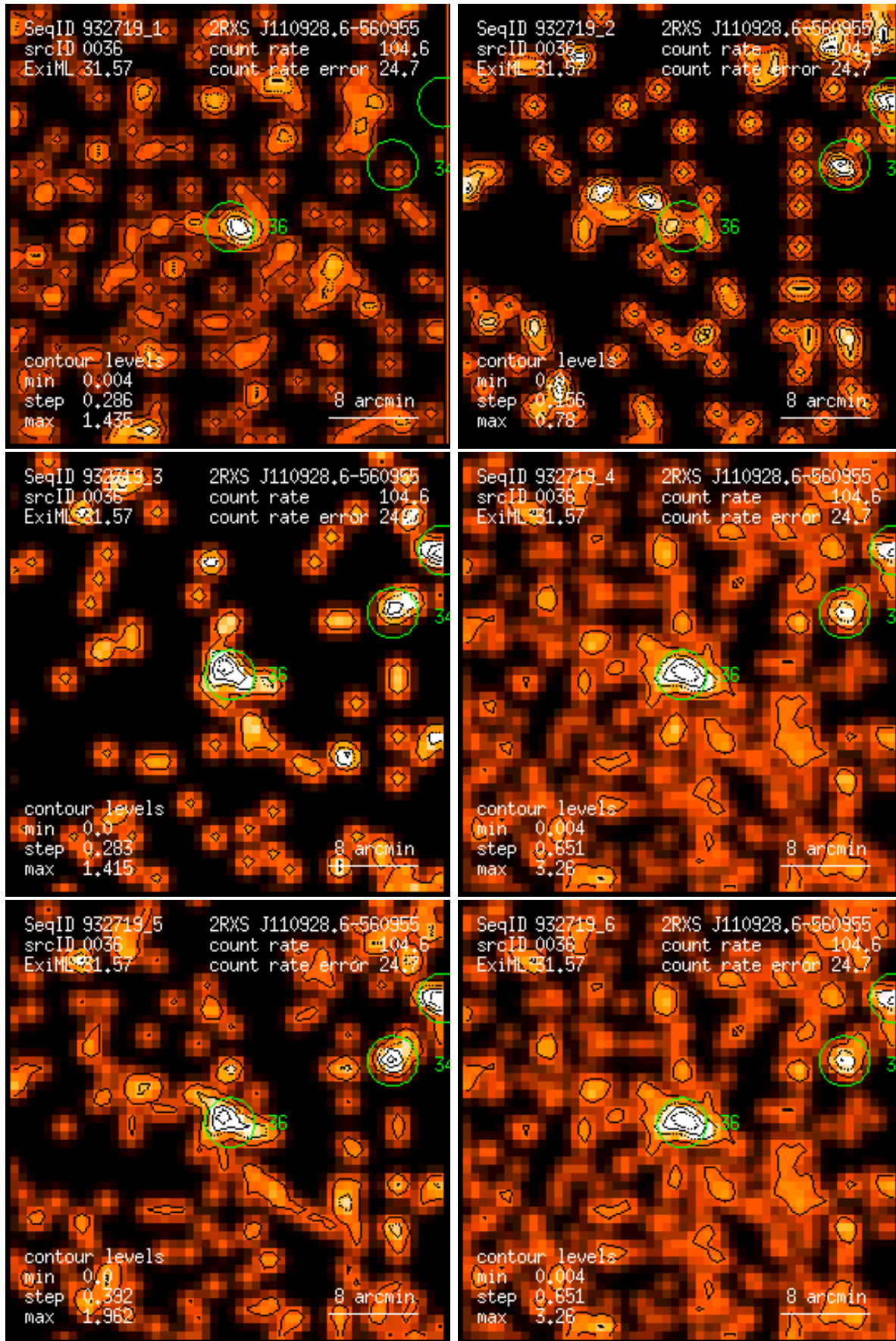
Figure 36: RASS 932719: detection 0036: band rate images, Gaussian filter: (1) PSPC channels 11 – 41, (2) 52 – 90, (3) 91 – 201, (4) 11 – 235, (5) 52 – 201, (6) 11 – 201. Broad band rates in counts/ks. Band rate contour levels in counts/ks/arcmin 2 .
