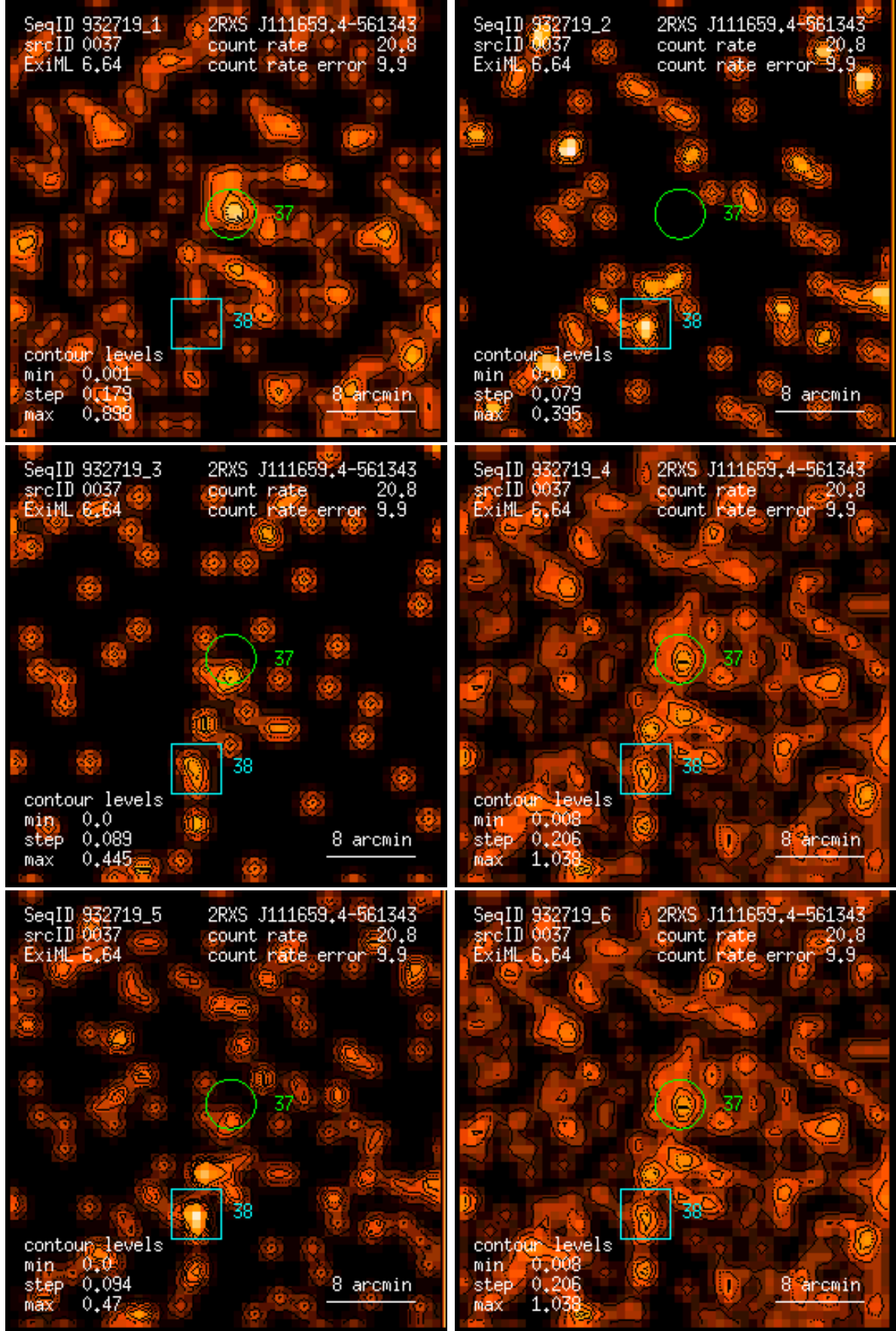
Figure 37: RASS 932719: detection 0037: band rate images, Gaussian filter: (1) PSPC channels 11 – 41, (2) 52 – 90, (3) 91 – 201, (4) 11 – 235, (5) 52 – 201, (6) 11 – 201. Broad band rates in counts/ks. Band rate contour levels in counts/ks/arcmin 2 .
