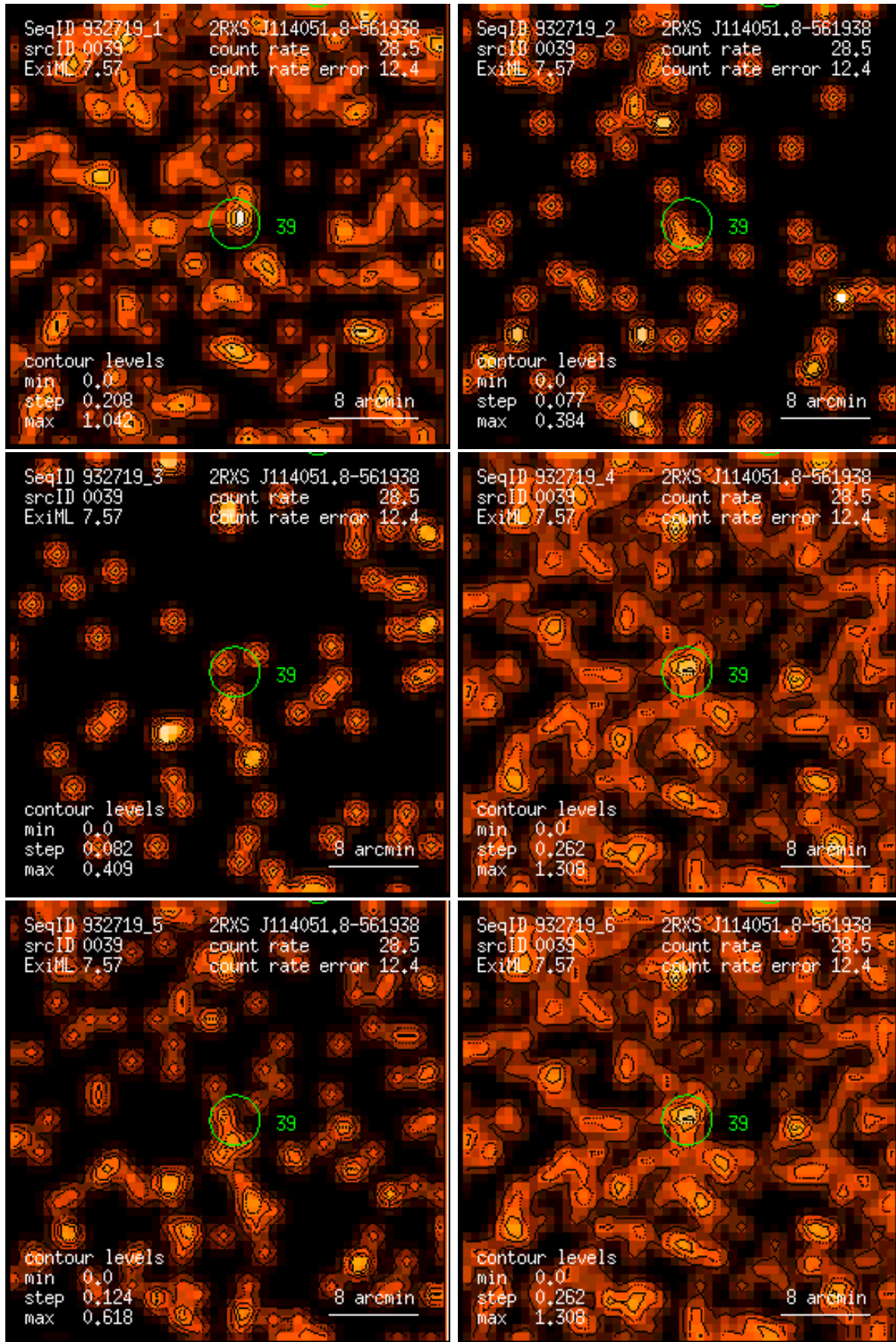
Figure 39: RASS 932719: detection 0039: band rate images, Gaussian filter: (1) PSPC channels 11 – 41, (2) 52 – 90, (3) 91 – 201, (4) 11 – 235, (5) 52 – 201, (6) 11 – 201. Broad band rates in counts/ks. Band rate contour levels in counts/ks/arcmin 2 .
