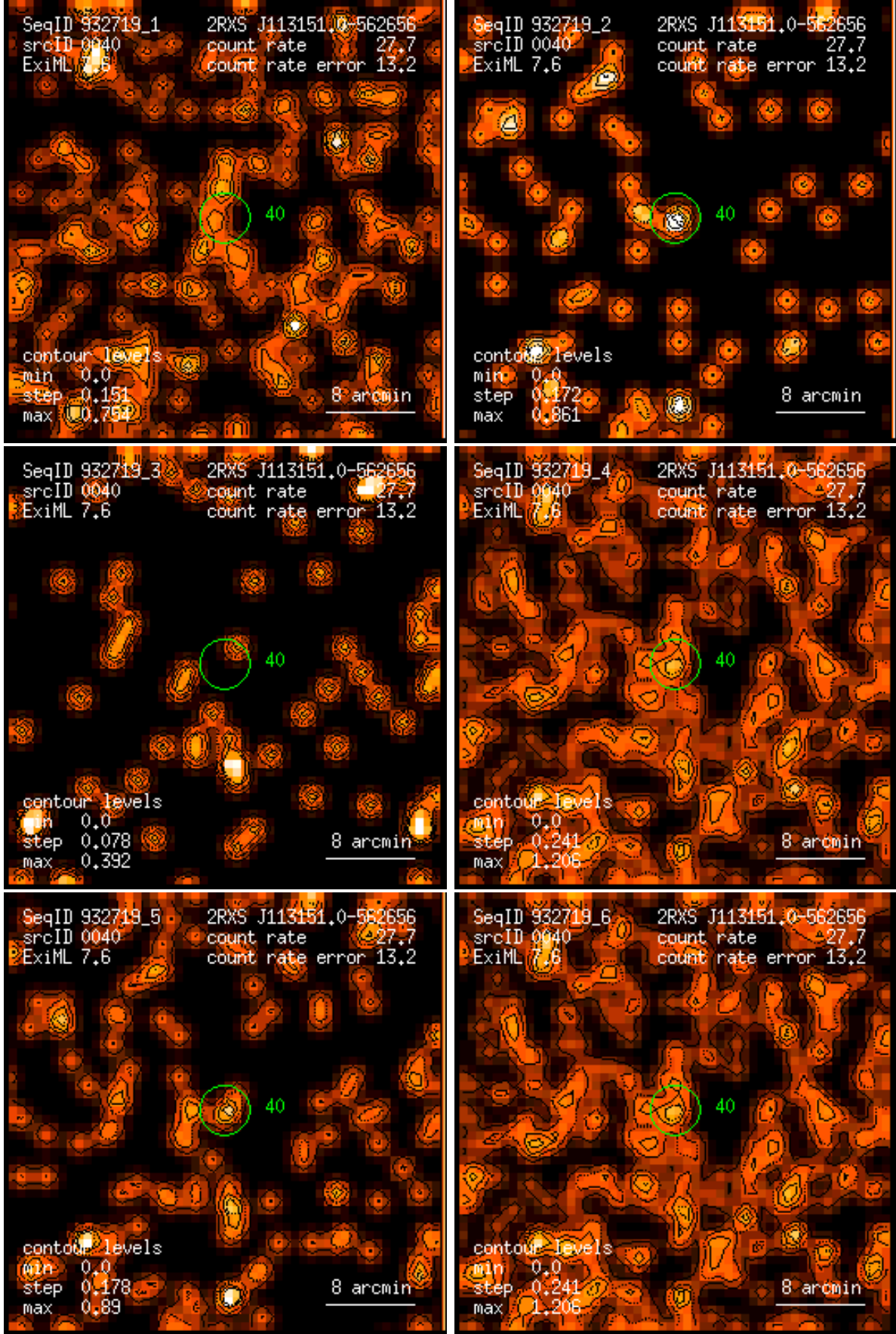
Figure 40: RASS 932719: detection 0040: band rate images, Gaussian filter: (1) PSPC channels 11 – 41, (2) 52 – 90, (3) 91 – 201, (4) 11 – 235, (5) 52 – 201, (6) 11 – 201. Broad band rates in counts/ks. Band rate contour levels in counts/ks/arcmin 2 .
