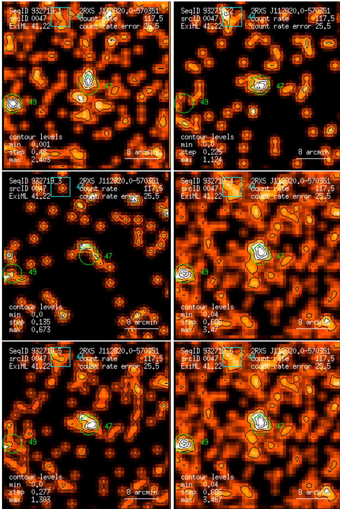
Figure 47: RASS 932719: detection 0047: band rate images, Gaussian filter: (1) PSPC channels 11 – 41, (2) 52 – 90, (3) 91 – 201, (4) 11 – 235, (5) 52 – 201, (6) 11 – 201. Broad band rates in counts/ks. Band rate contour levels in counts/ks/arcmin 2 .
