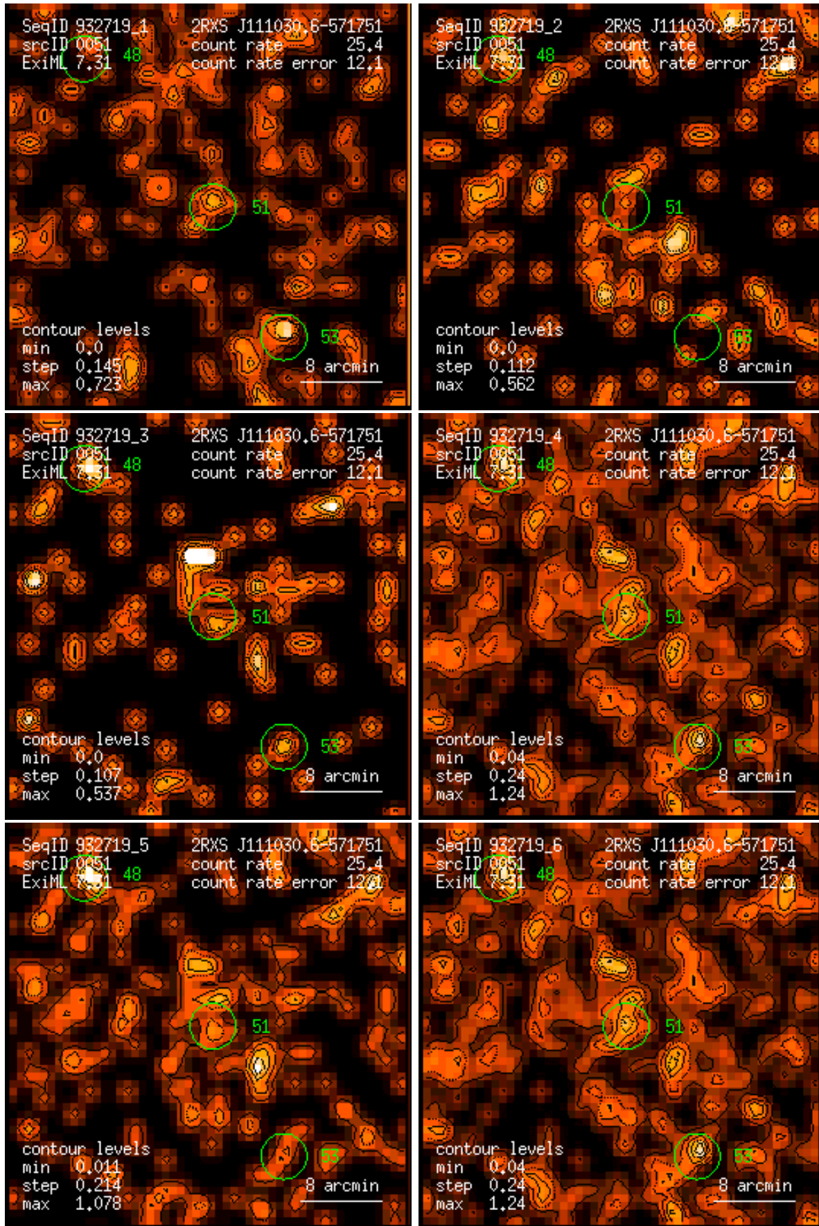
Figure 51: RASS 932719: detection 0051: band rate images, Gaussian filter: (1) PSPC channels 11 – 41, (2) 52 – 90, (3) 91 – 201, (4) 11 – 235, (5) 52 – 201, (6) 11 – 201. Broad band rates in counts/ks. Band rate contour levels in counts/ks/arcmin 2 .
