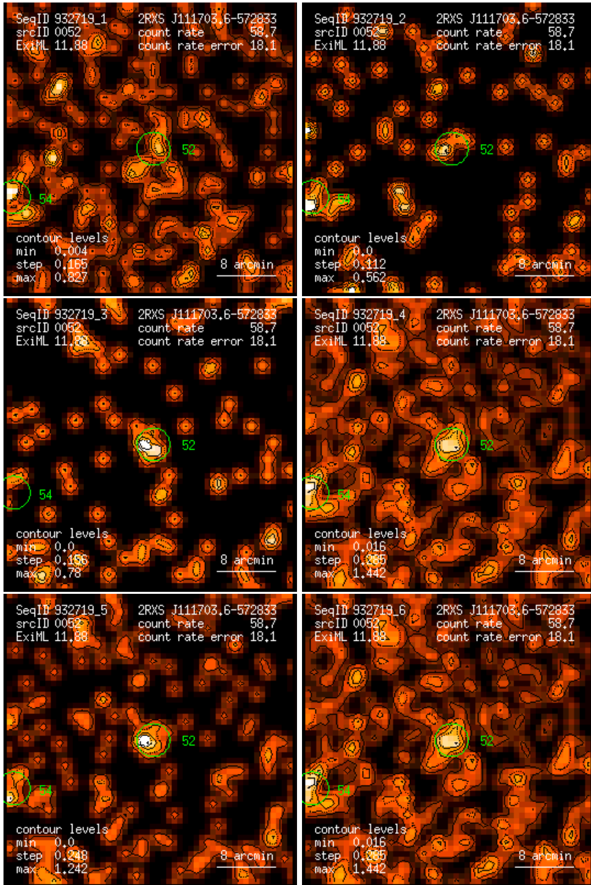
Figure 52: RASS 932719: detection 0052: band rate images, Gaussian filter: (1) PSPC channels 11 – 41, (2) 52 – 90, (3) 91 – 201, (4) 11 – 235, (5) 52 – 201, (6) 11 – 201. Broad band rates in counts/ks. Band rate contour levels in counts/ks/arcmin 2 .
