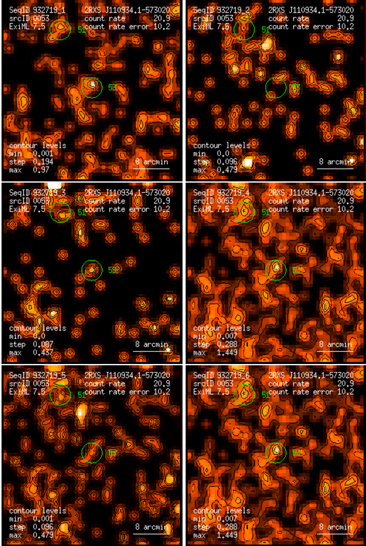
Figure 53: RASS 932719: detection 0053: band rate images, Gaussian filter: (1) PSPC channels 11 – 41, (2) 52 – 90, (3) 91 – 201, (4) 11 – 235, (5) 52 – 201, (6) 11 – 201. Broad band rates in counts/ks. Band rate contour levels in counts/ks/arcmin 2 .
