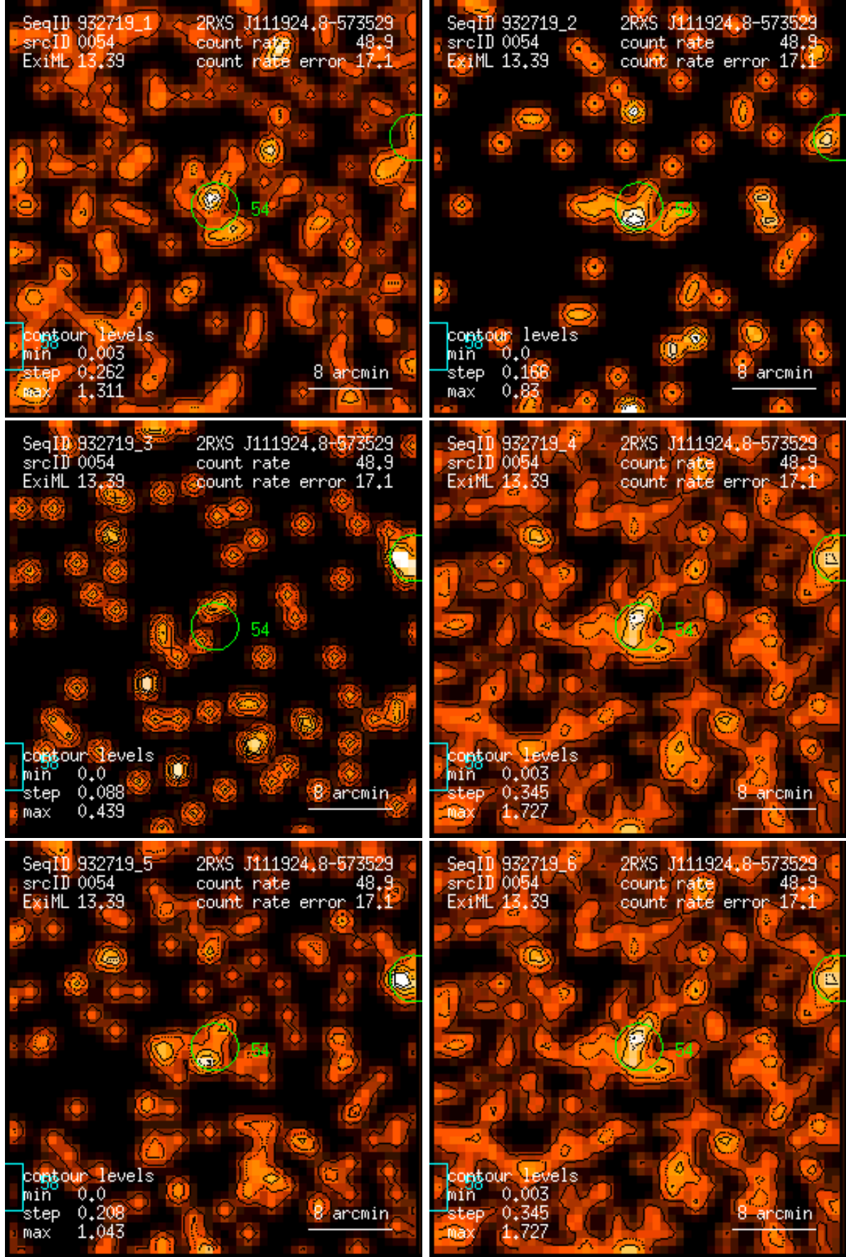
Figure 54: RASS 932719: detection 0054: band rate images, Gaussian filter: (1) PSPC channels 11 – 41, (2) 52 – 90, (3) 91 – 201, (4) 11 – 235, (5) 52 – 201, (6) 11 – 201. Broad band rates in counts/ks. Band rate contour levels in counts/ks/arcmin 2 .
