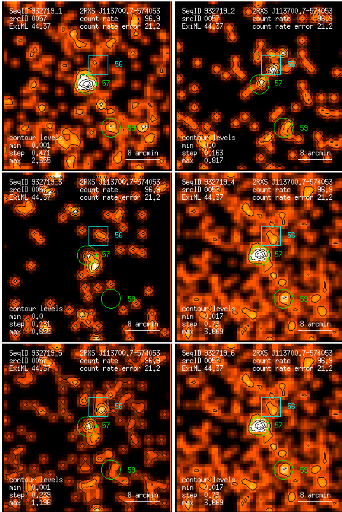
Figure 57: RASS 932719: detection 0057: band rate images, Gaussian filter: (1) PSPC channels 11 – 41, (2) 52 – 90, (3) 91 – 201, (4) 11 – 235, (5) 52 – 201, (6) 11 – 201. Broad band rates in counts/ks. Band rate contour levels in counts/ks/arcmin 2 .
