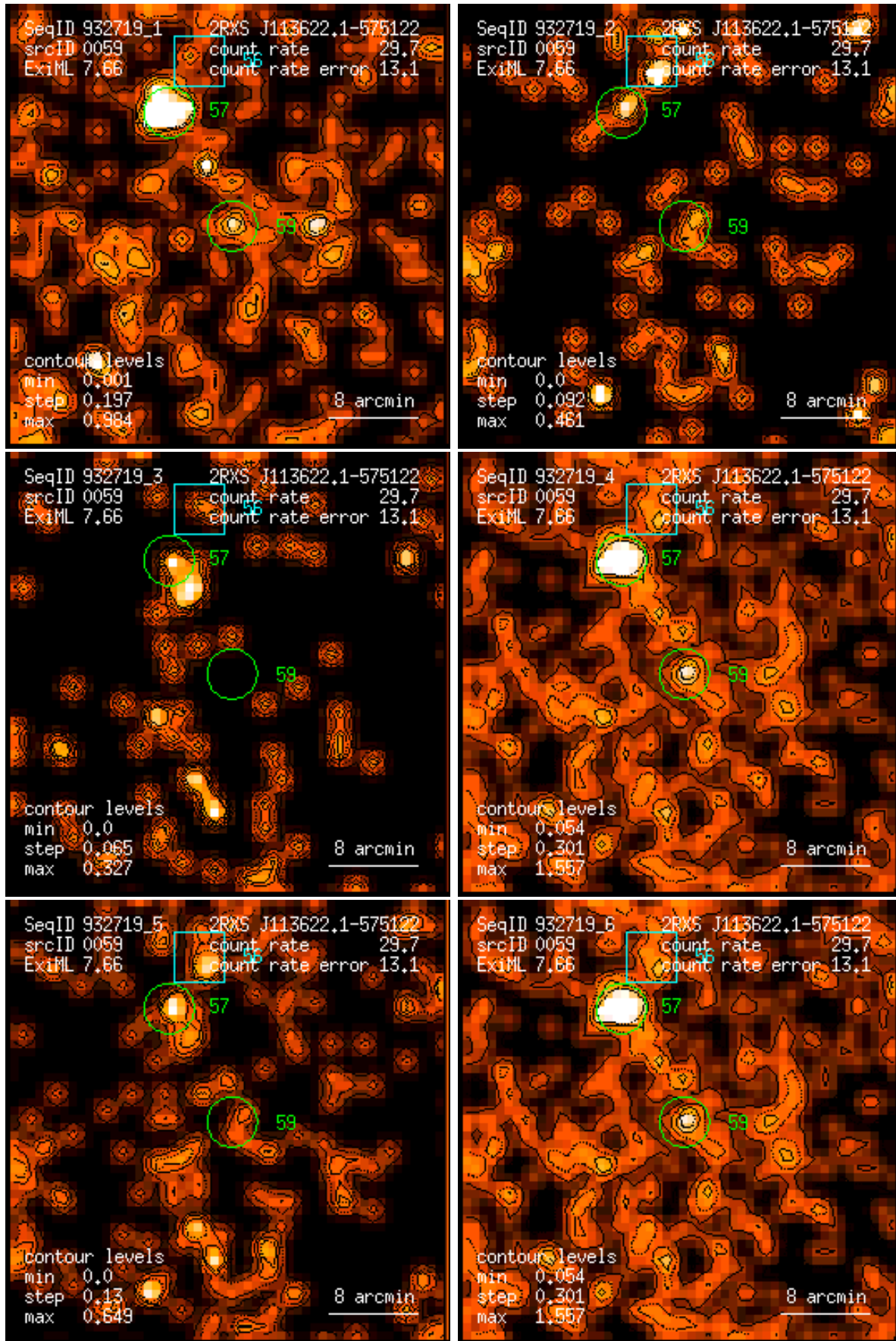
Figure 59: RASS 932719: detection 0059: band rate images, Gaussian filter: (1) PSPC channels 11 – 41, (2) 52 – 90, (3) 91 – 201, (4) 11 – 235, (5) 52 – 201, (6) 11 – 201. Broad band rates in counts/ks. Band rate contour levels in counts/ks/arcmin 2 .
