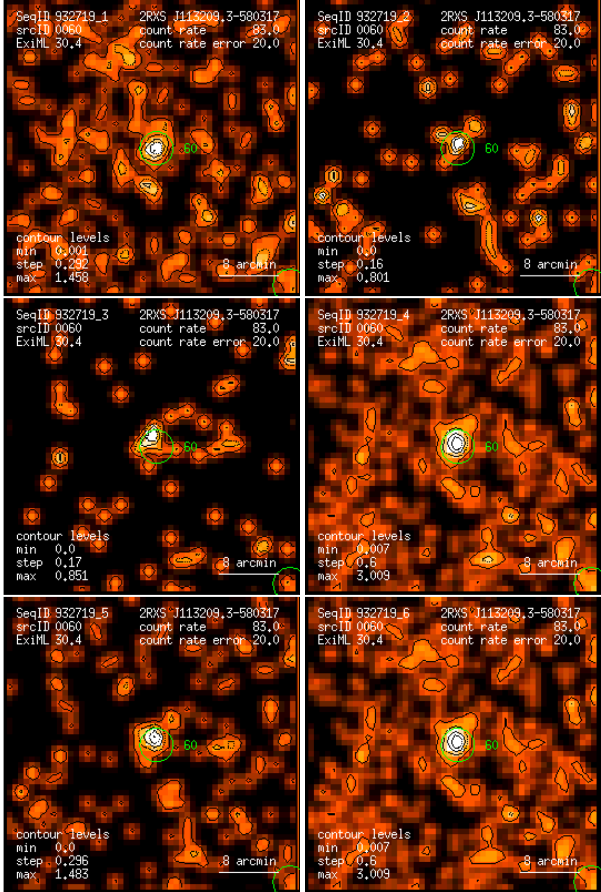
Figure 60: RASS 932719: detection 0060: band rate images, Gaussian filter: (1) PSPC channels 11 – 41, (2) 52 – 90, (3) 91 – 201, (4) 11 – 235, (5) 52 – 201, (6) 11 – 201. Broad band rates in counts/ks. Band rate contour levels in counts/ks/arcmin 2 .
