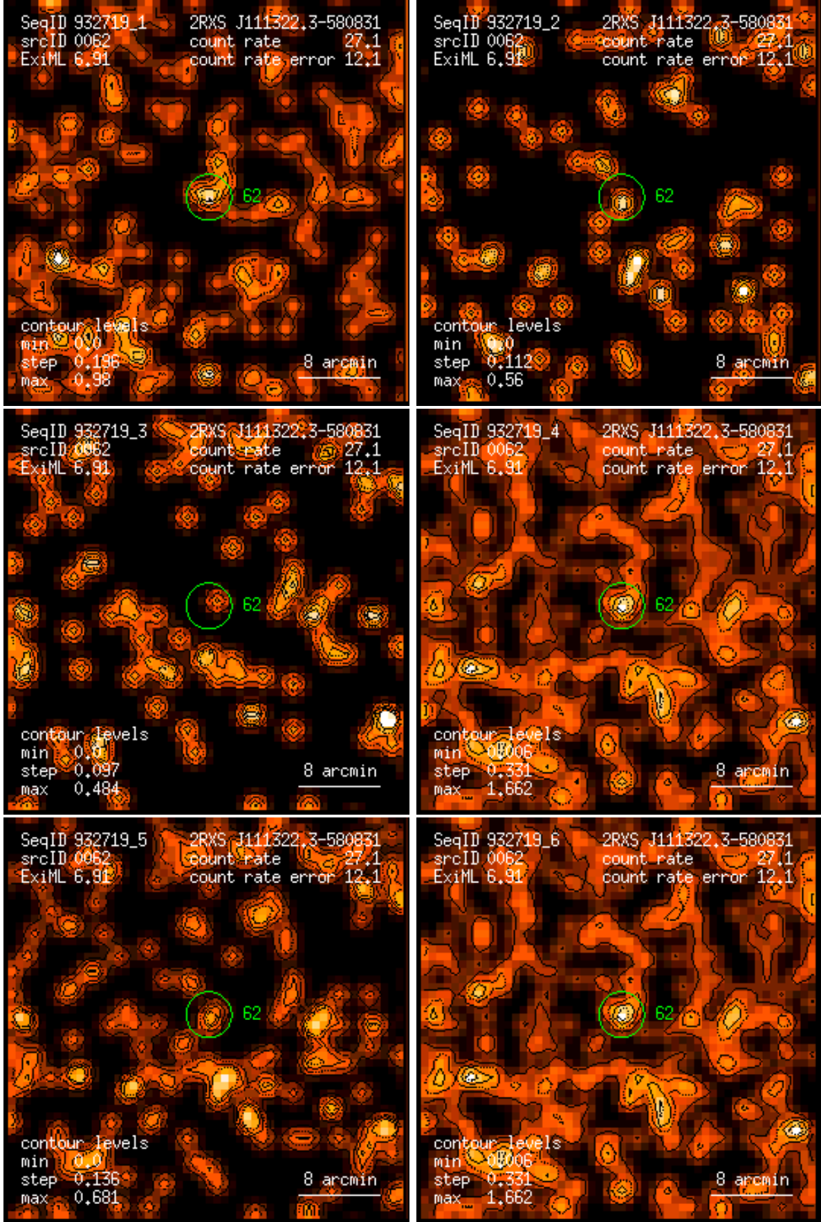
Figure 62: RASS 932719: detection 0062: band rate images, Gaussian filter: (1) PSPC channels 11 – 41, (2) 52 – 90, (3) 91 – 201, (4) 11 – 235, (5) 52 – 201, (6) 11 – 201. Broad band rates in counts/ks. Band rate contour levels in counts/ks/arcmin 2 .
