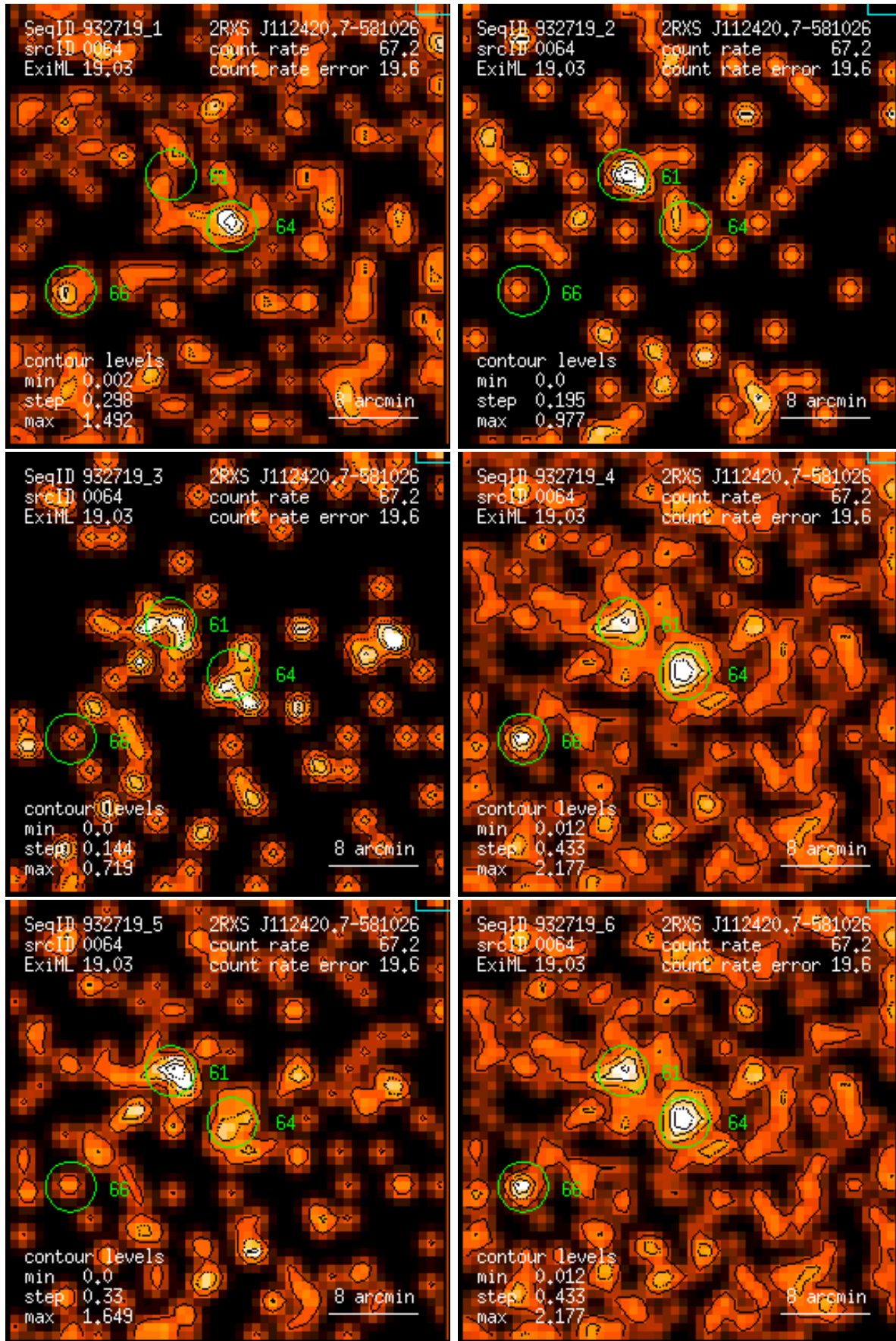
Figure 64: RASS 932719: detection 0064: band rate images, Gaussian filter: (1) PSPC channels 11 – 41, (2) 52 – 90, (3) 91 – 201, (4) 11 – 235, (5) 52 – 201, (6) 11 – 201. Broad band rates in counts/ks. Band rate contour levels in counts/ks/arcmin 2 .
