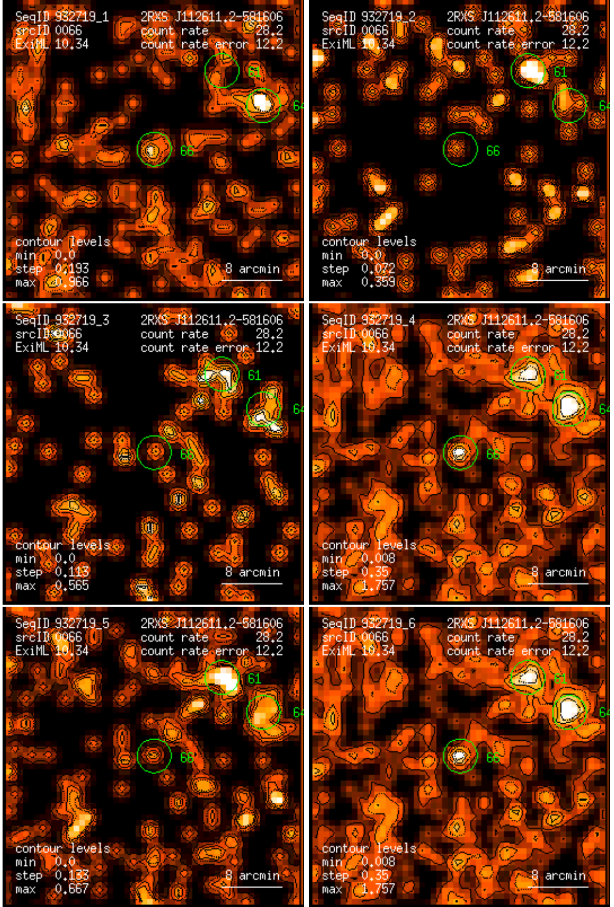
Figure 66: RASS 932719: detection 0066: band rate images, Gaussian filter: (1) PSPC channels 11 – 41, (2) 52 – 90, (3) 91 – 201, (4) 11 – 235, (5) 52 – 201, (6) 11 – 201. Broad band rates in counts/ks. Band rate contour levels in counts/ks/arcmin 2 .
