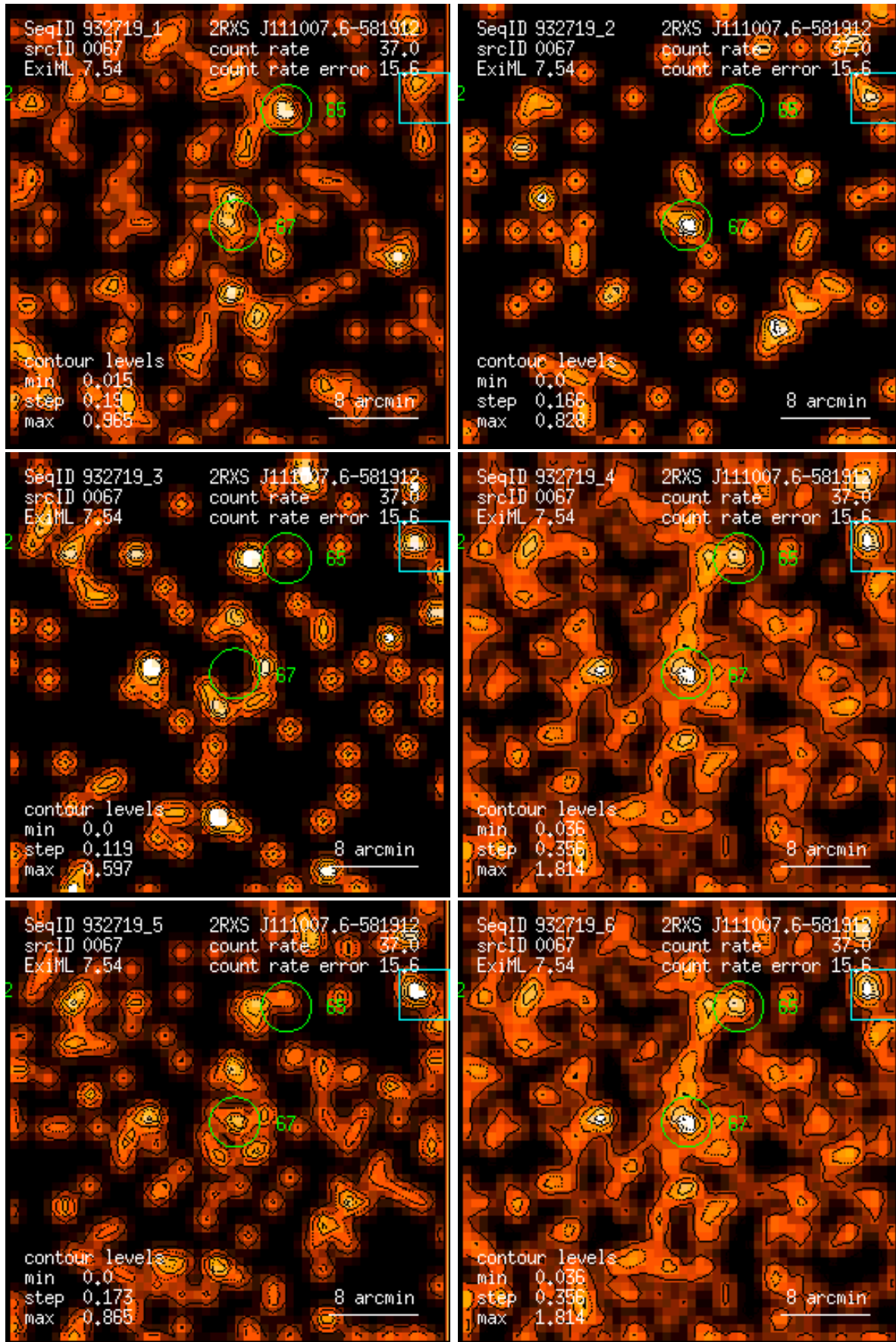
Figure 67: RASS 932719: detection 0067: band rate images, Gaussian filter: (1) PSPC channels 11 – 41, (2) 52 – 90, (3) 91 – 201, (4) 11 – 235, (5) 52 – 201, (6) 11 – 201. Broad band rates in counts/ks. Band rate contour levels in counts/ks/arcmin 2 .
