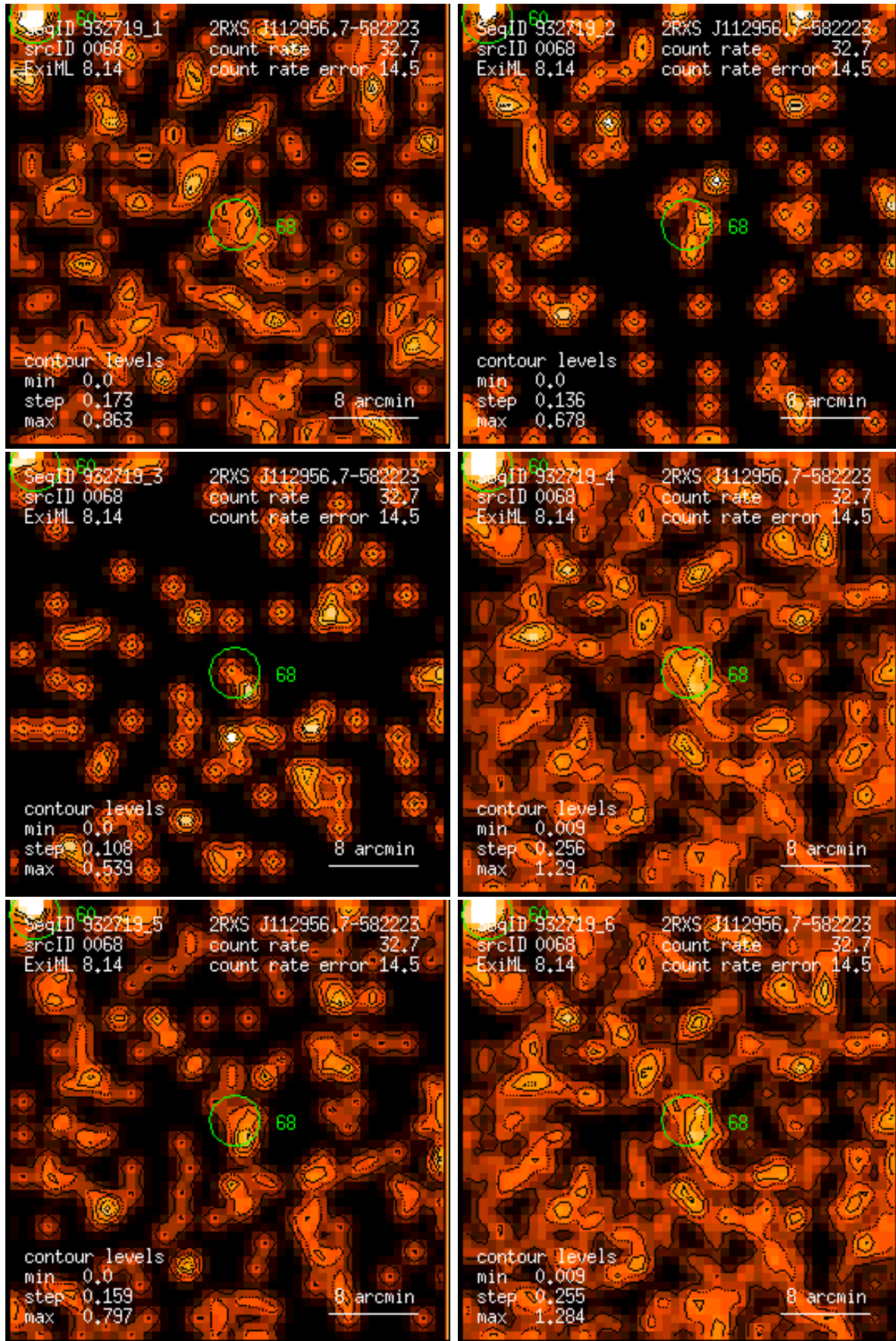
Figure 68: RASS 932719: detection 0068: band rate images, Gaussian filter: (1) PSPC channels 11 – 41, (2) 52 – 90, (3) 91 – 201, (4) 11 – 235, (5) 52 – 201, (6) 11 – 201. Broad band rates in counts/ks. Band rate contour levels in counts/ks/arcmin 2 .
