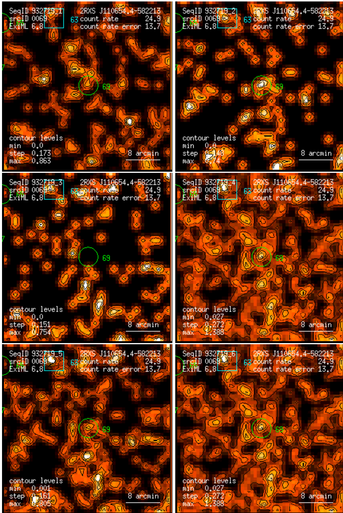
Figure 69: RASS 932719: detection 0069: band rate images, Gaussian filter: (1) PSPC channels 11 – 41, (2) 52 – 90, (3) 91 – 201, (4) 11 – 235, (5) 52 – 201, (6) 11 – 201. Broad band rates in counts/ks. Band rate contour levels in counts/ks/arcmin 2 .
