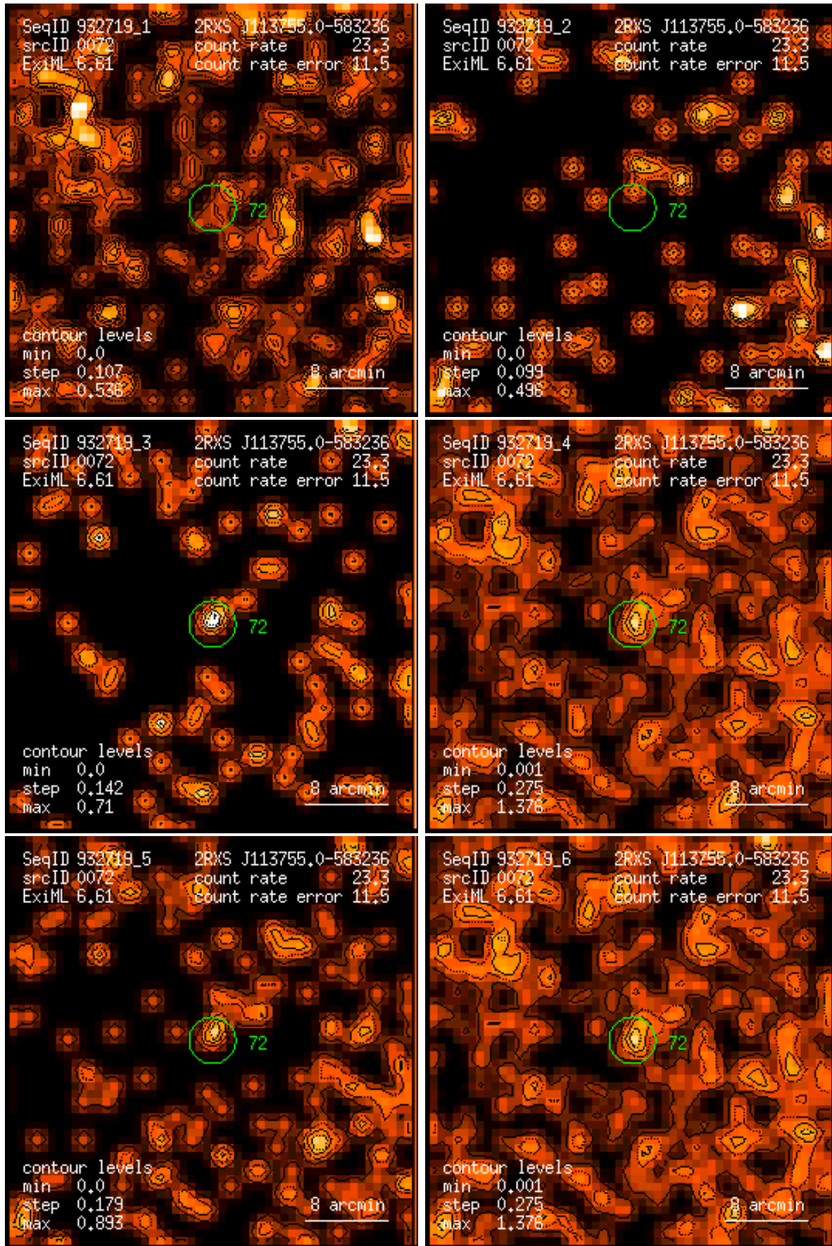
Figure 72: RASS 932719: detection 0072: band rate images, Gaussian filter: (1) PSPC channels 11 – 41, (2) 52 – 90, (3) 91 – 201, (4) 11 – 235, (5) 52 – 201, (6) 11 – 201. Broad band rates in counts/ks. Band rate contour levels in counts/ks/arcmin 2 .
